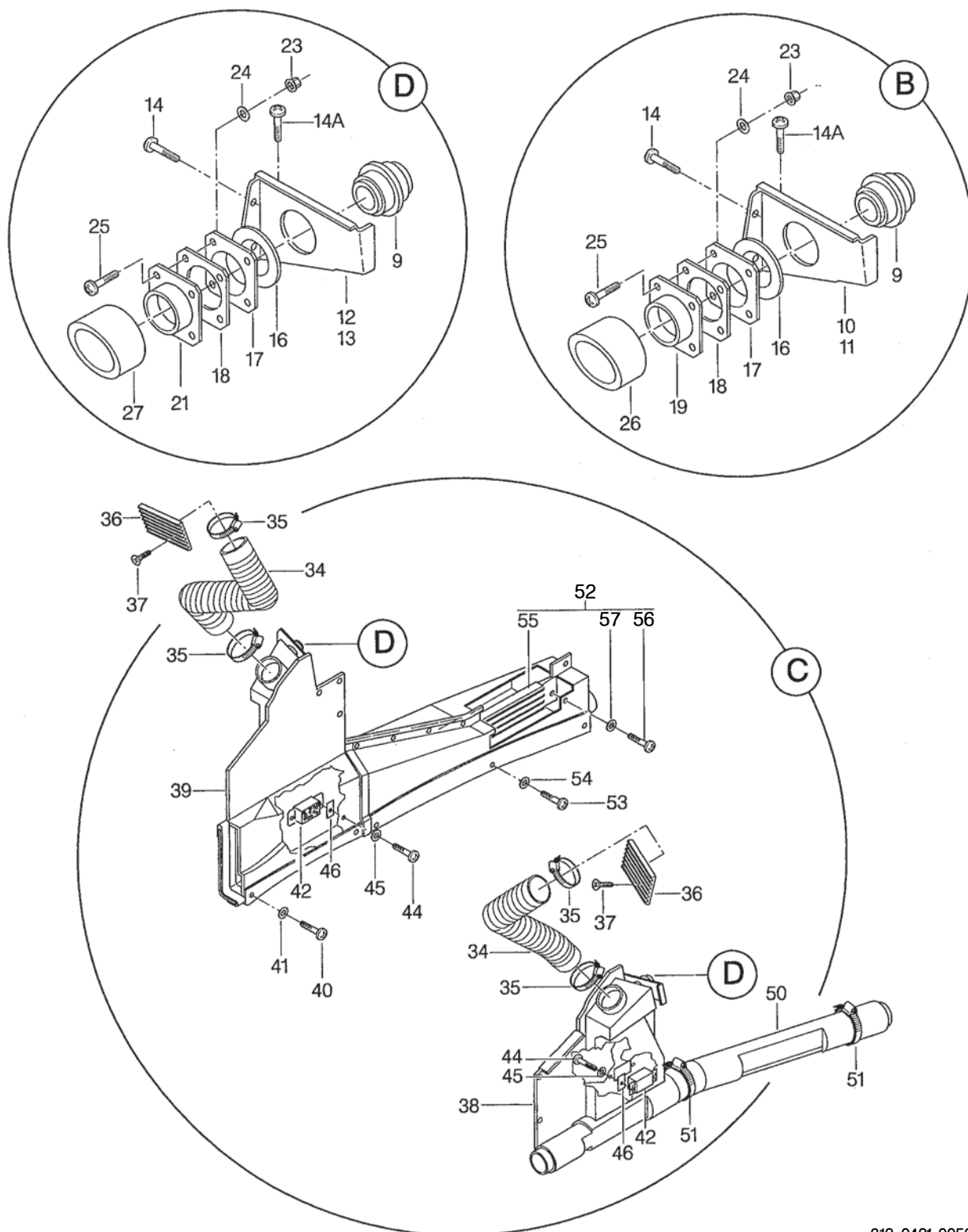
FIGURA 03. DISTRIBUICAO DE AR CONDICIONADO INSTL (FOLHA 2 DE 3) FIGURE 03. AIR CONDITIONING DISTRIBUTION INSTL (SHEET 2 OF 3)
