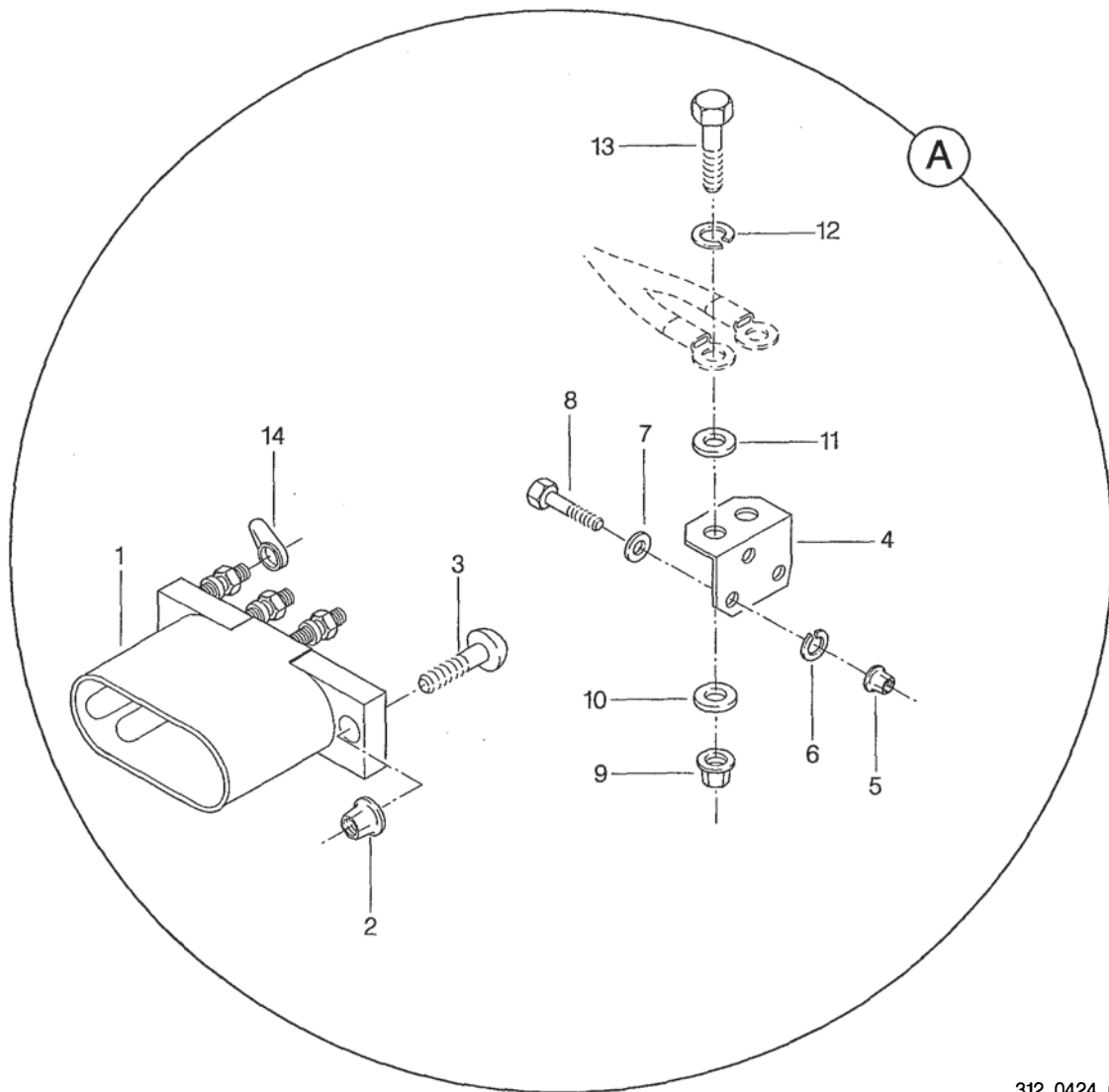
FIGURA 01. TOMADA DE FONTE EXTERNA INSTL FIGURE 01. EXTERNAL POWER RECEPTACLE INSTL
