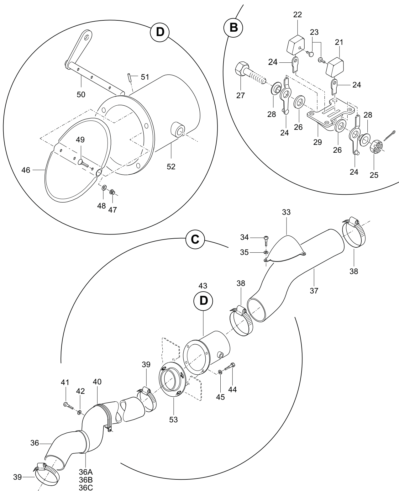
FIGURA 15. VENTILACAO/AQUECIMENTO D A CABINE INSTL (FOLHA 2 D E 3) FIGURE 15. COCKPIT HEATING/VENTILATION SYSTEM INSTL (SHEET 2 OF 3)
