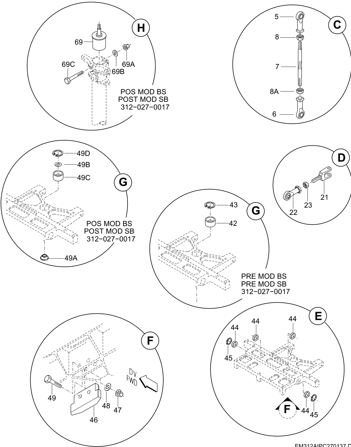
FIGURA 01.CONJUNTO DO PEDAL INST (FOLHA 3 DE 3) FIGURE 01. PEDALS INST (SHEET 3 OF 3)
