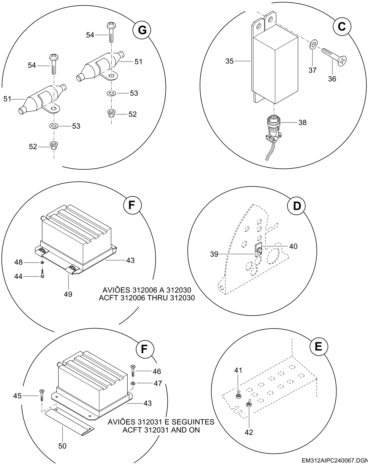
FIGURA 01. BATERIA E ACESSORIOS INSTL (FOLHA 3 DE 4) FIGURE 01. BATTERY & ACESSORIES INSTL (SHEET 3 OF 4)
