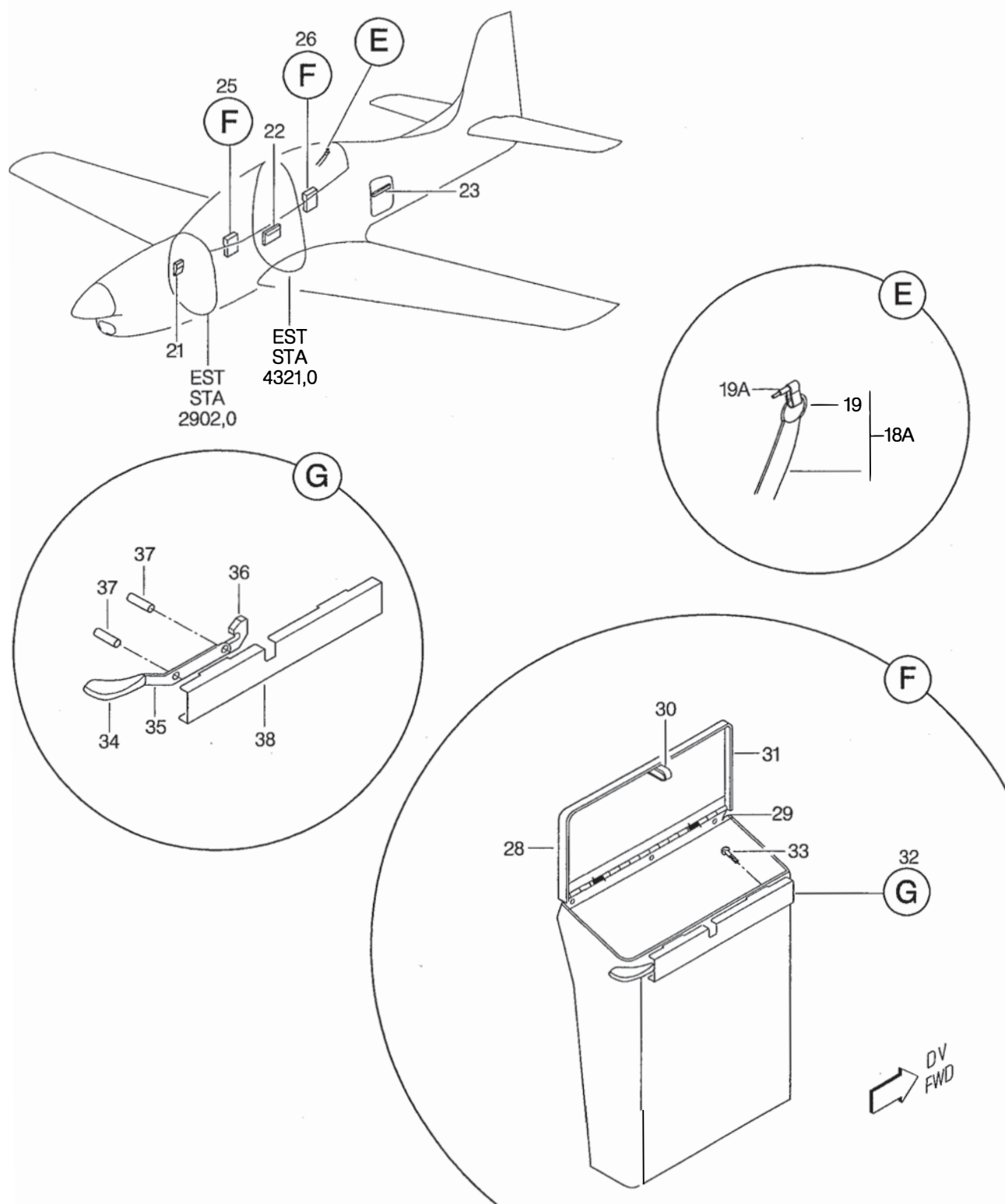
FIGURA 02. ACESSORIOS BASICOS INSTL (FOLHA 2 DE 2) FIGURE 02. BASIC EQUIPMENT INSTL (SHEET 2 OF 2)
