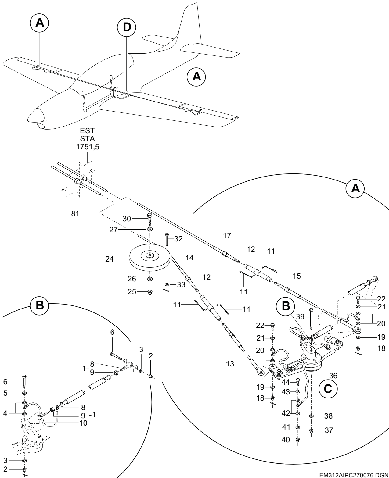
FIGURA 02. COMANDO DO AILERON (FOLHA 1 DE 2) FIGURE 02. AILERON CONTROL INST, WINGS (SHEET 1 OF 2)
