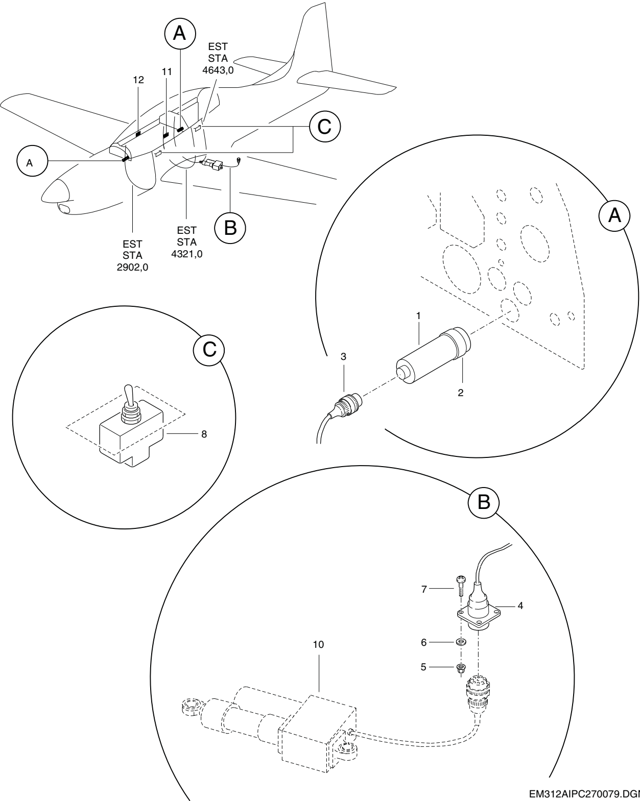
FIGURA 01. SISTEMA DE INDICACAO INSTL, COMPENSADOR DO AILERON FIGURE 01. POSITION INDICATING SYSTEM INSTL, AILERON TRIM TAB
