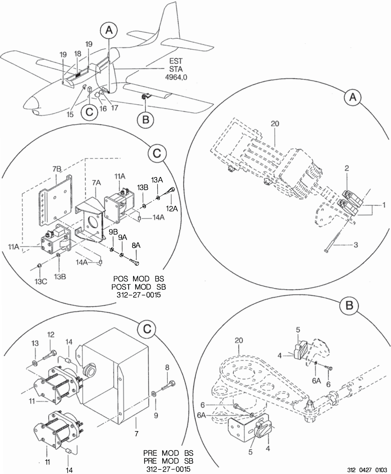
FIGURA 01. INDICACAO DE COMANDO INSTL, FLAPES FIGURE 01. CONTROL INDICATING INSTL, FLAP
