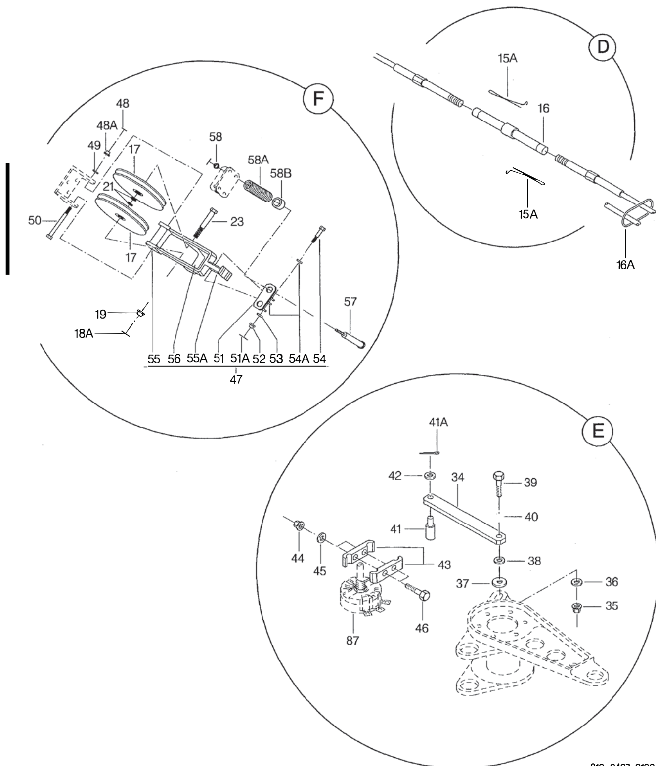
FIGURA 01. INTERLIGACAO DOS FLAPES INSTL (FOLHA 2 DE 2) FIGURE 01. FLAPS INTERCONNECTION INSTL (SHEET 2 OF 2)
