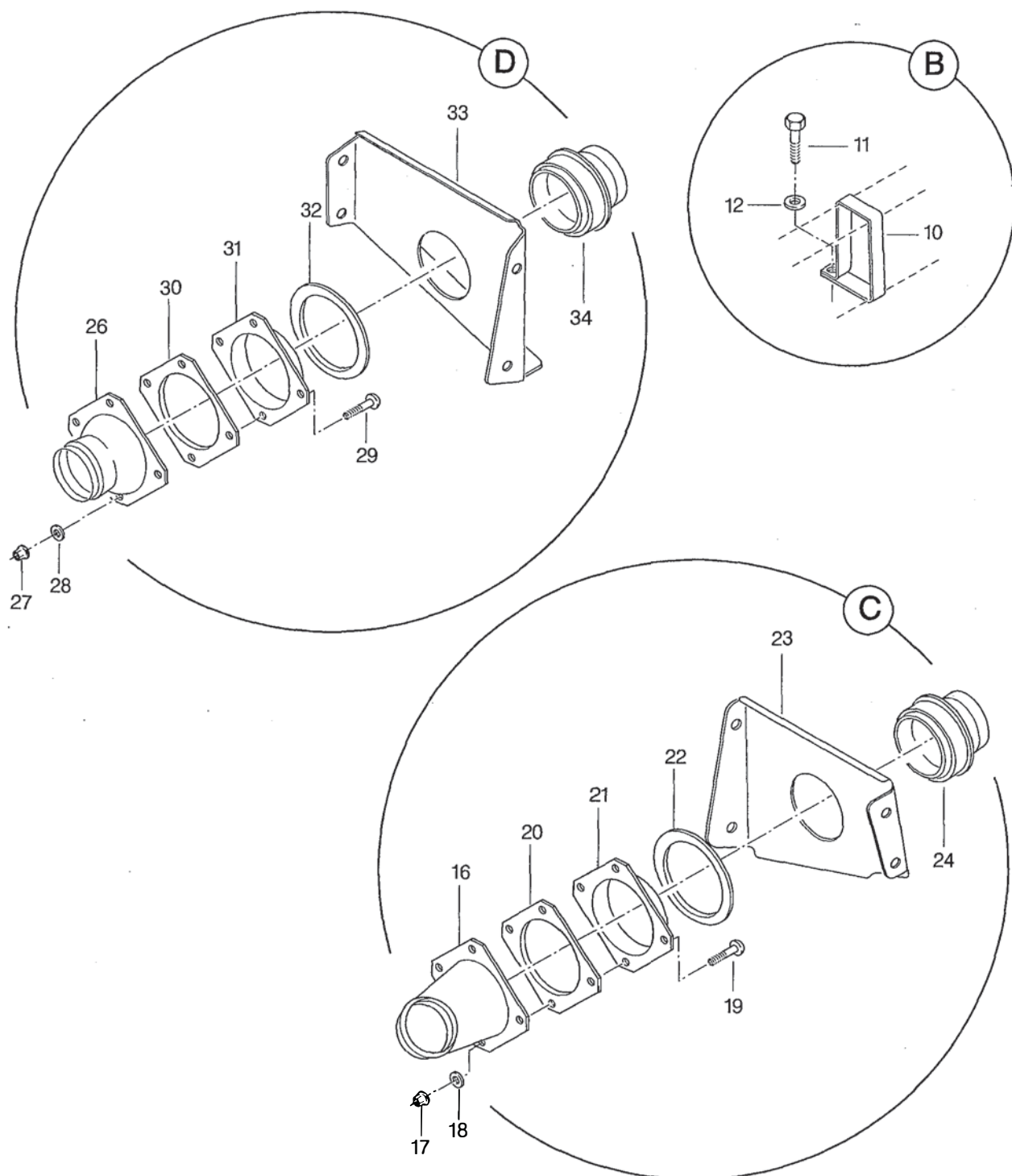
FIGURA 06. DISTRIBUICAO DE AR CONDICIONADO INSTL, POSTO DIANTEIRO (FOLHA 2 DE 2) FIGURE 06. AIR CONDITIONING DISTRIBUTION INSTL, FRONT FLIGHT STATION (SHEET 2 OF 2)
