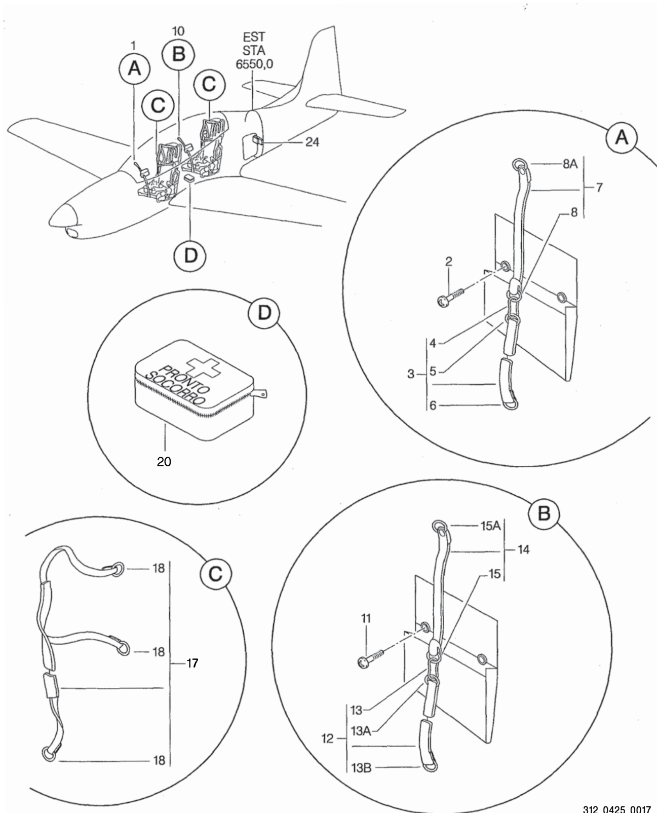
FIGURA 02. ACESSORIOS BASICOS INSTL (FOLHA 1 DE 2) FIGURE 02. BASIC EQUIPMENT INSTL (SHEET 1 OF 2)
