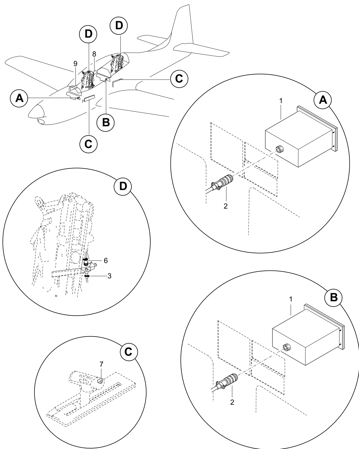
FIGURA 01. SISTEMA DE AUDIO INSTL FIGURE 01. AUDIO SYSTEM INSTL
