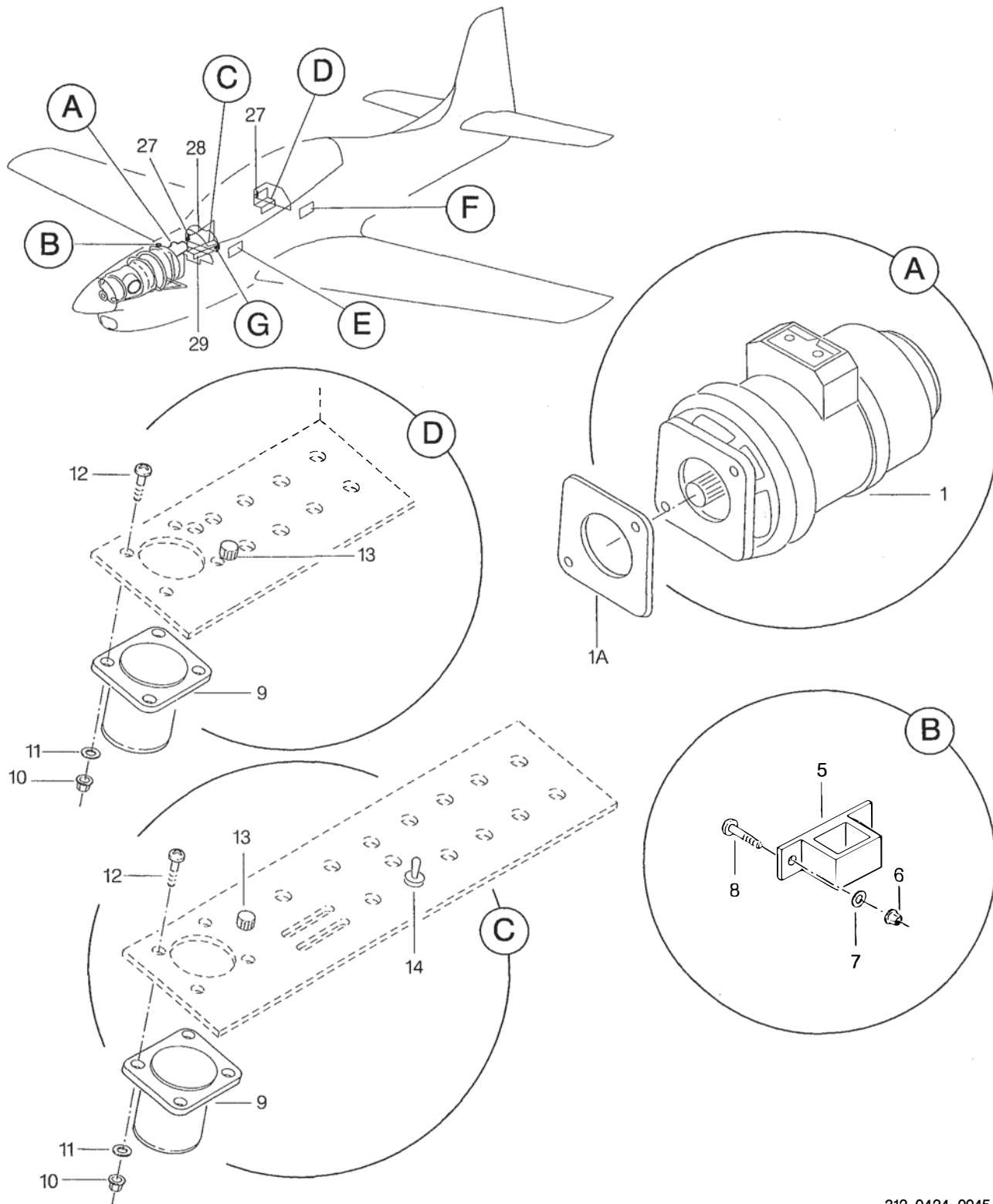
FIGURA 01. SISTEMA DE GERACAO DE CORRENTE CONTINUA INSTL (FOLHA 1 DE 2) FIGURE 01. DIRECT CURRENT GENERATION SYSTEM INSTL (SHEET 1 OF 2)
