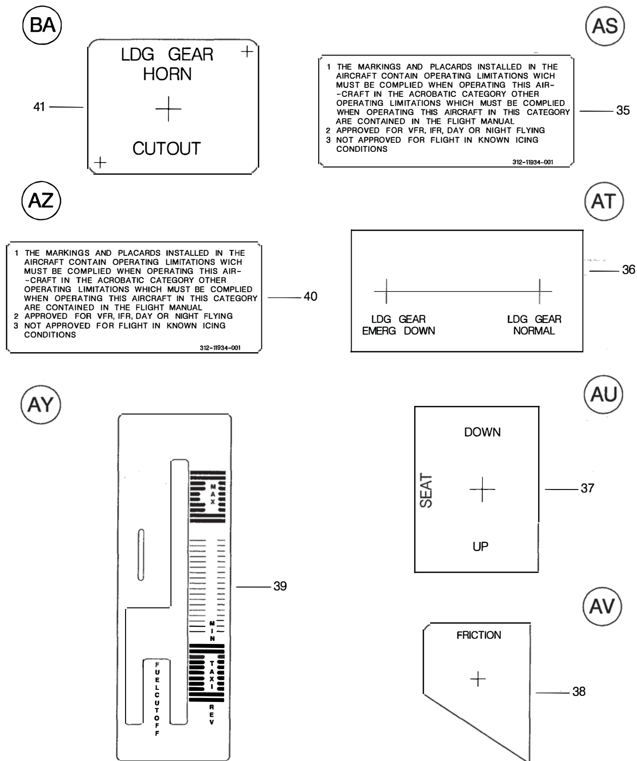
FIGURA 02. INSCRICOES E MARCACOES INTERNAS INSTL (FOLHA 8 DE 13) FIGURE 02. INTERIOR PLACARDS & MARKINGS INSTL (SHEET 8 OF 13)
