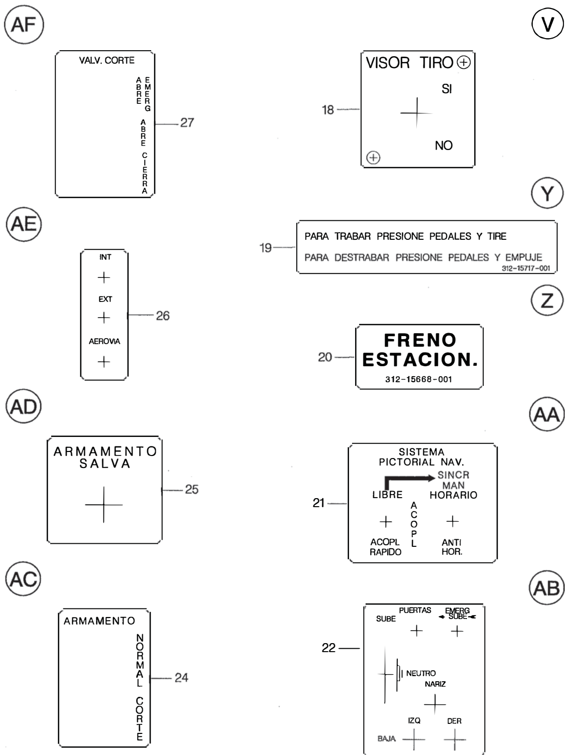
FIGURA 05. INSCRICOES E MARCACOES INTERNAS INSTL (FOLHA 5 DE 12) FIGURE 05. INTERIOR PLACARDS & MARKINGS INSTL (SHEET 5 OF 12)
