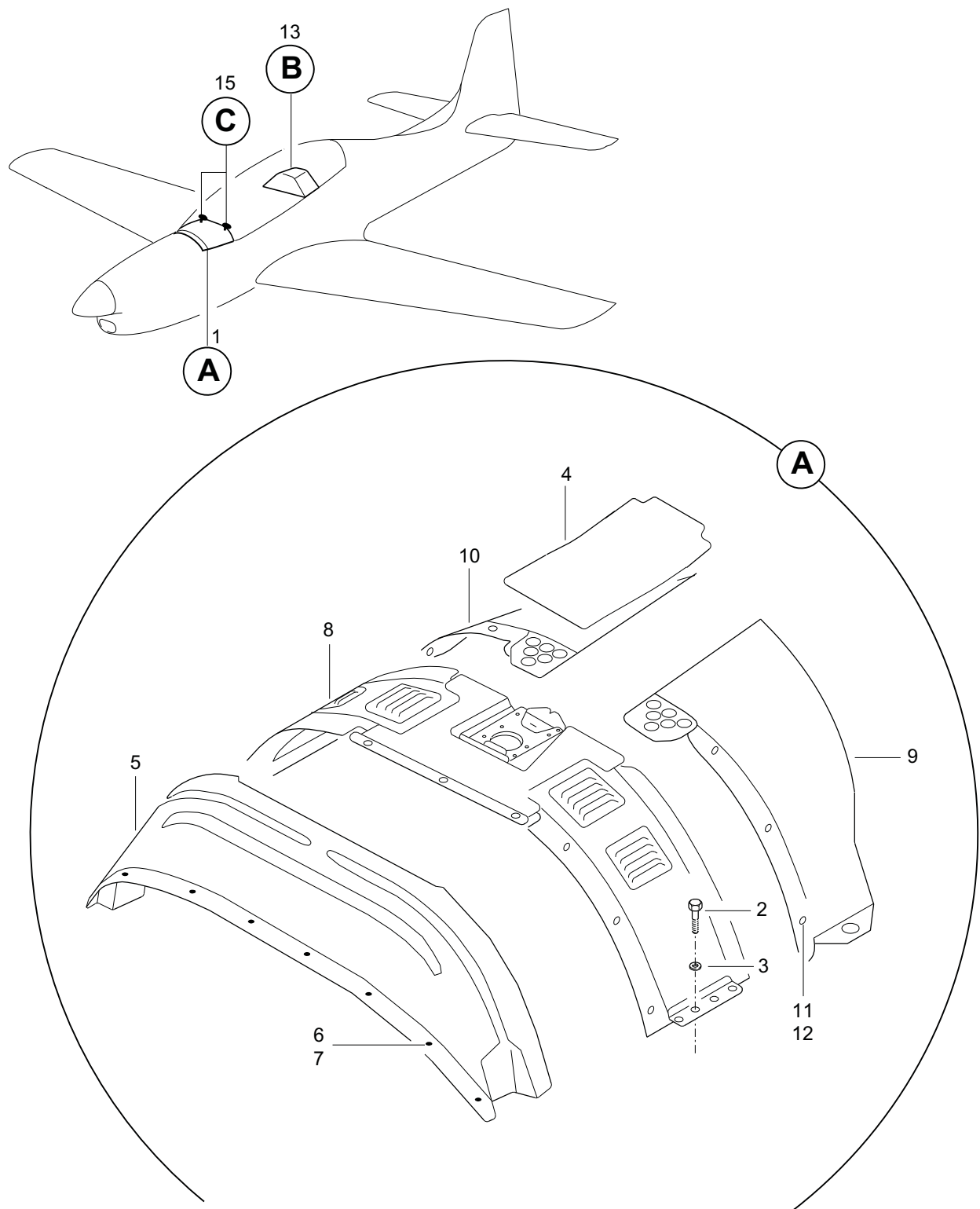
FIGURA 01. PALAS DE PROTECAO INSTL (FOLHA 1 DE 2) FIGURE 01. GLARESHIELDS INSTL (SHEET 1 OF 2)
