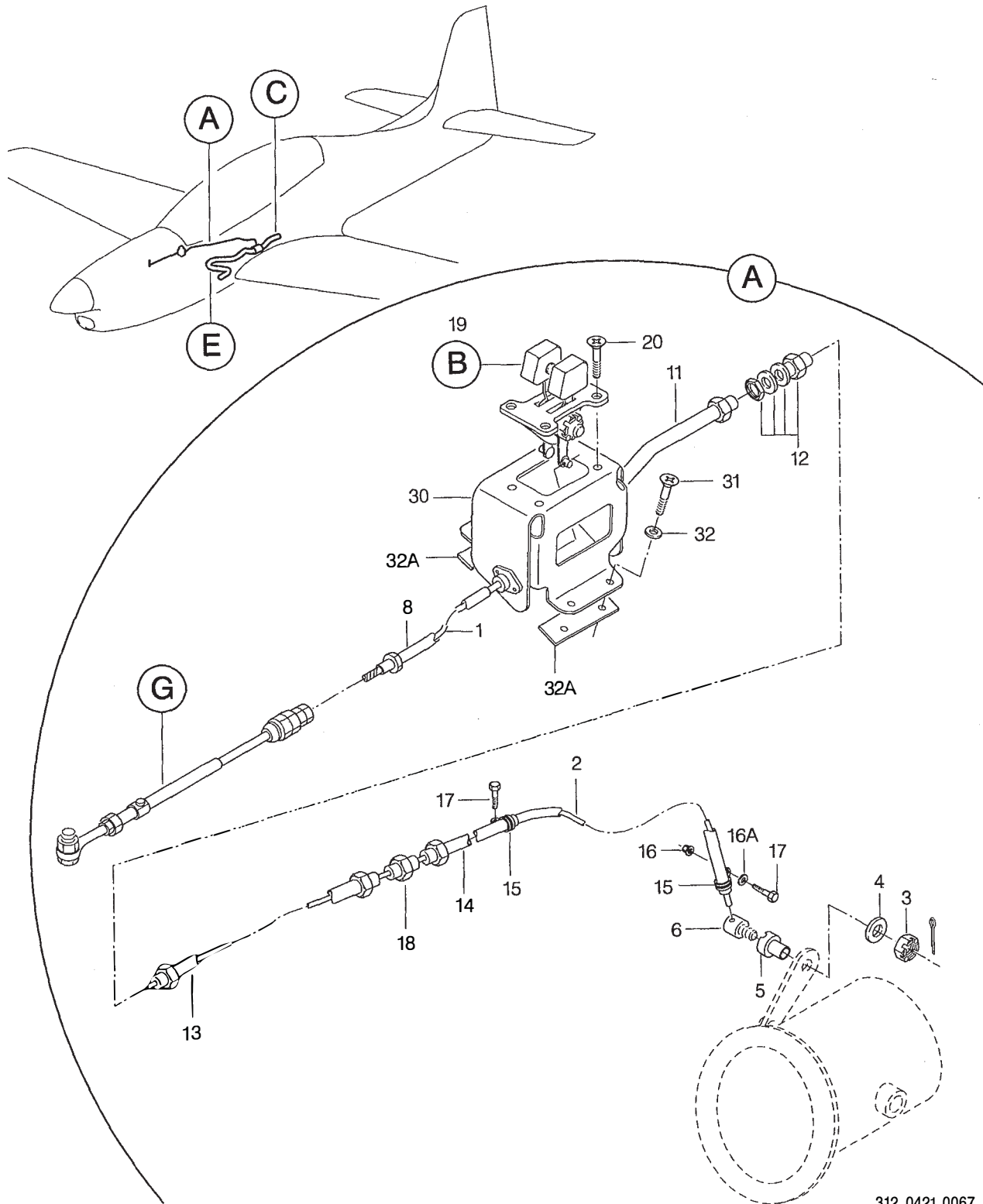
FIGURA 15. VENTILACAO/AQUECIMENTO D A CABINE INSTL (FOLHA 1 D E 3) FIGURE 15. COCKPIT HEATING/VENTILATION SYSTEM INSTL (SHEET 1 OF 3)
