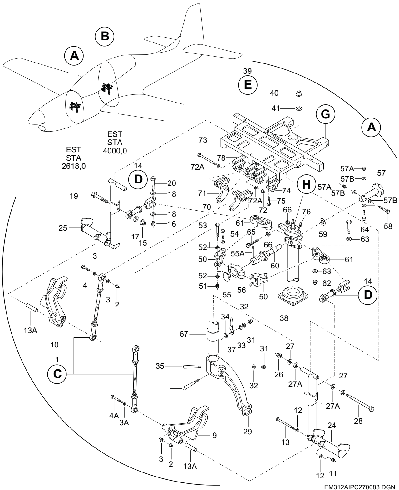
FIGURA 01.CONJUNTO DO PEDAL INST (FOLHA 1 DE 3) FIGURE 01. PEDALS INST (SHEET 1 OF 3)
