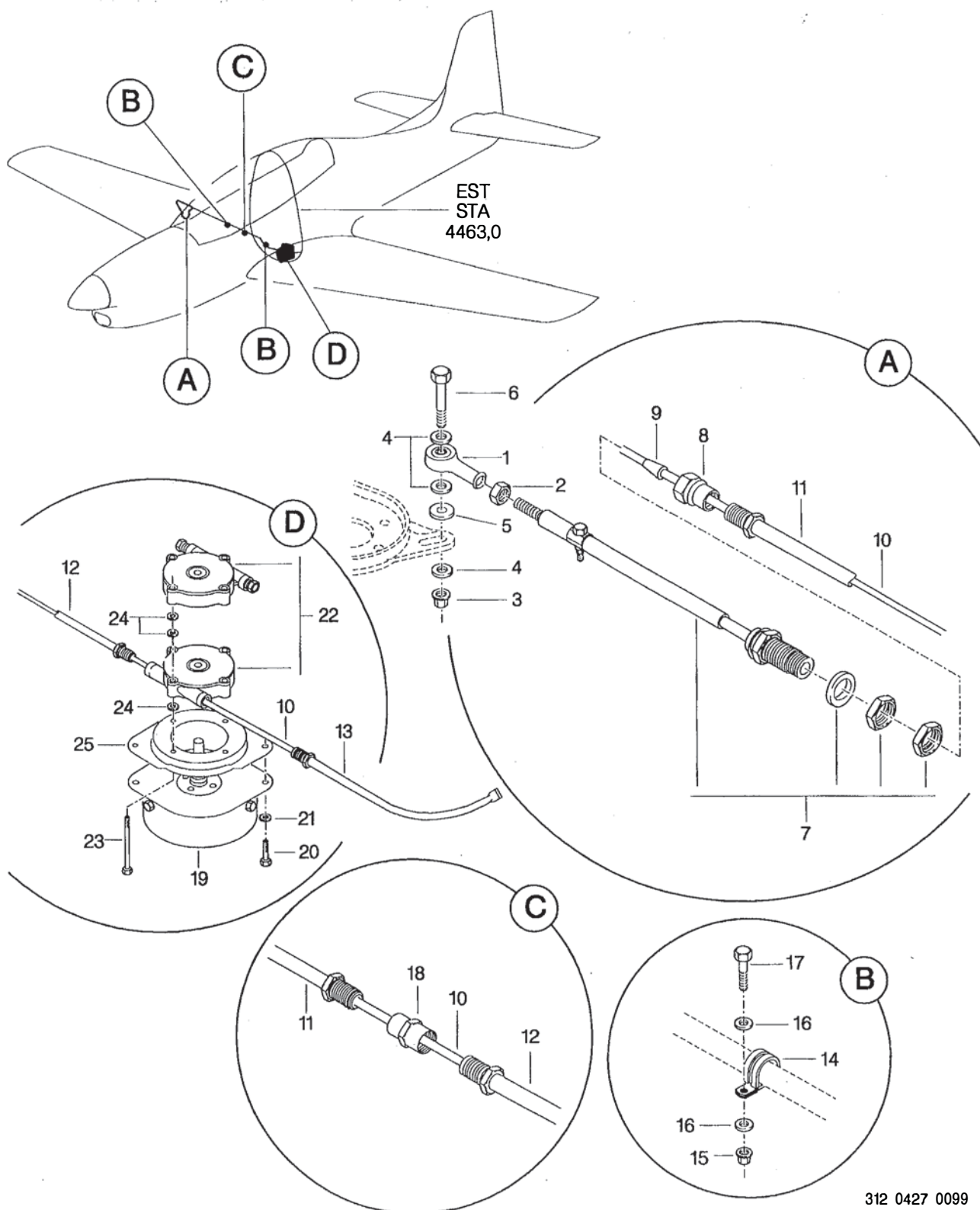
FIGURA 01. CONTROLE DOS FLAPES INSTL FIGURE 01. FLAP POSITION CONTROL INSTL
