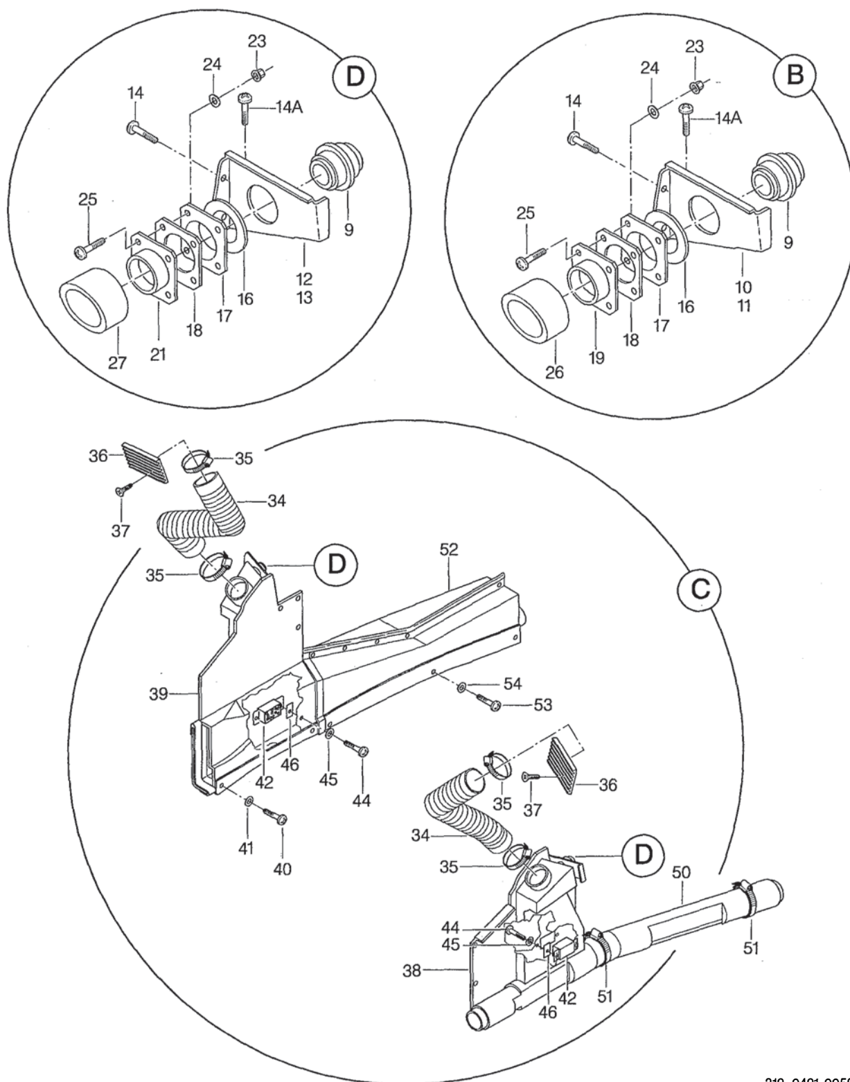
FIGURA 04. DISTRIBUICAO DE AR CONDICIONADO INSTL (FOLHA 2 DE 3) FIGURE 04. AIR CONDITIONING DISTRIBUTION INSTL (SHEET 2 OF 3)
