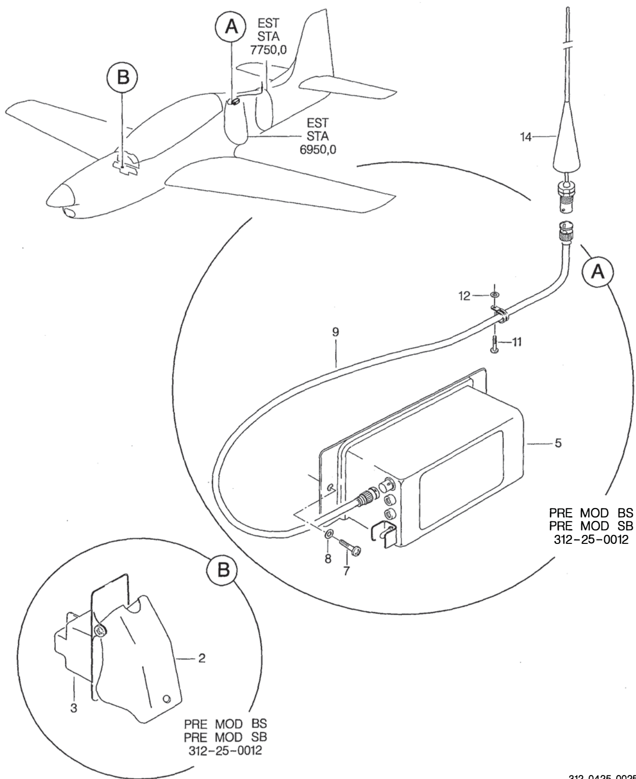
FIGURA 01. TRANSMISSOR DE EMERGENCIA INSTL (FOLHA 1 DE 2) FIGURE 01. EMERGENCY LOCATOR TRANSMITTER INSTL (SHEET 1 OF 2)
