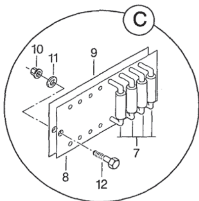
FIGURA 02. CONTROLE DO AR CONDICIONADO INSTL (FOLHA 1 DE 2) FIGURE 02. AIR CONDITIONING CONTROL SYSTEM INSTL (SHEET 1 OF 2)
