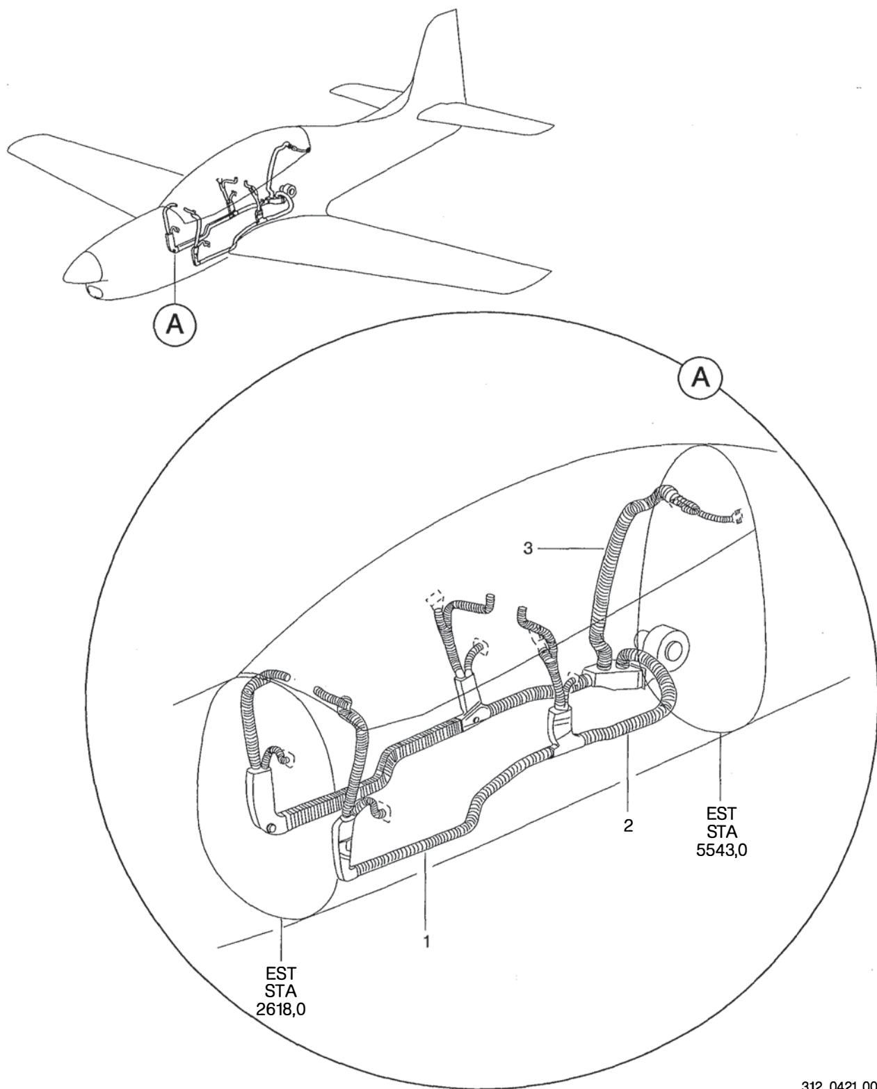
FIGURA 05. DISTRIBUICAO DE AR CONDICIONADO INSTL FIGURE 05. AIR CONDITIONING DISTRIBUTION INSTL
