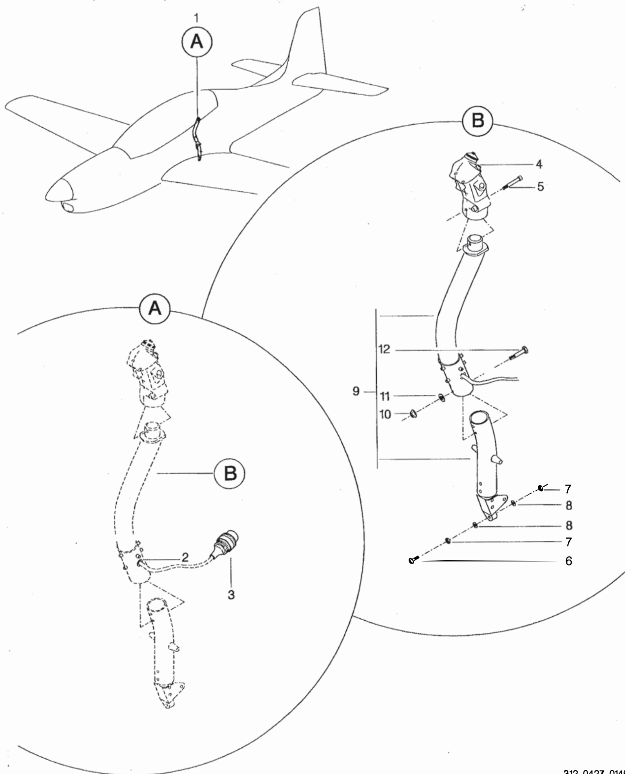
FIGURA 02. MANCHES CONJ FIGURE 02. CONTROL STICKS ASSY
