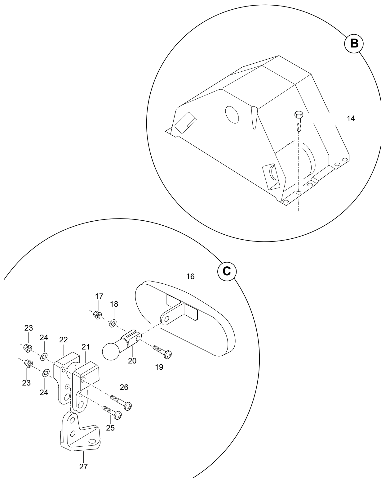
FIGURA 01. PALAS DE PROTECAO INSTL (FOLHA 2 DE 2) FIGURE 01. GLARESHIELDS INSTL (SHEET 2 OF 2)
