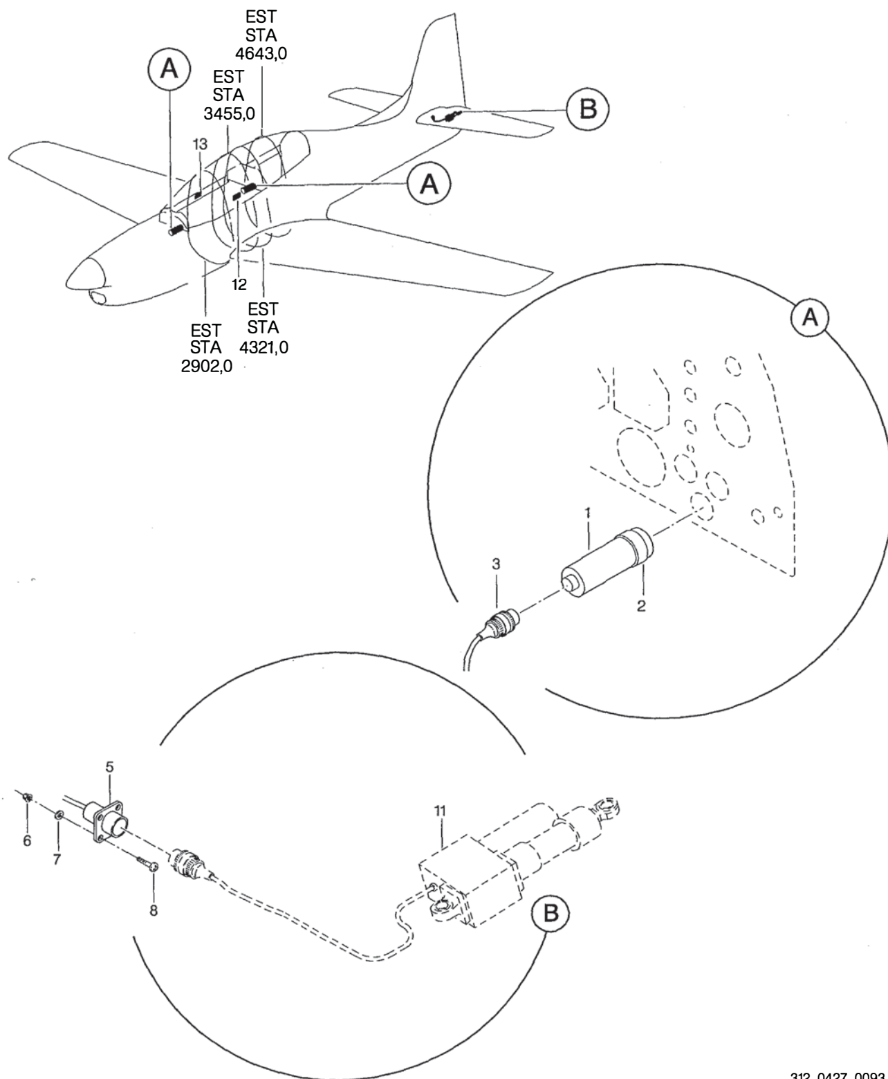
FIGURA 01. SISTEMA DE INDICACAO INSTL, COMPENSADOR INSTL FIGURE 01. POSITION INDICATING SYSTEM INSTL, ELEVATOR TRIM TAB
