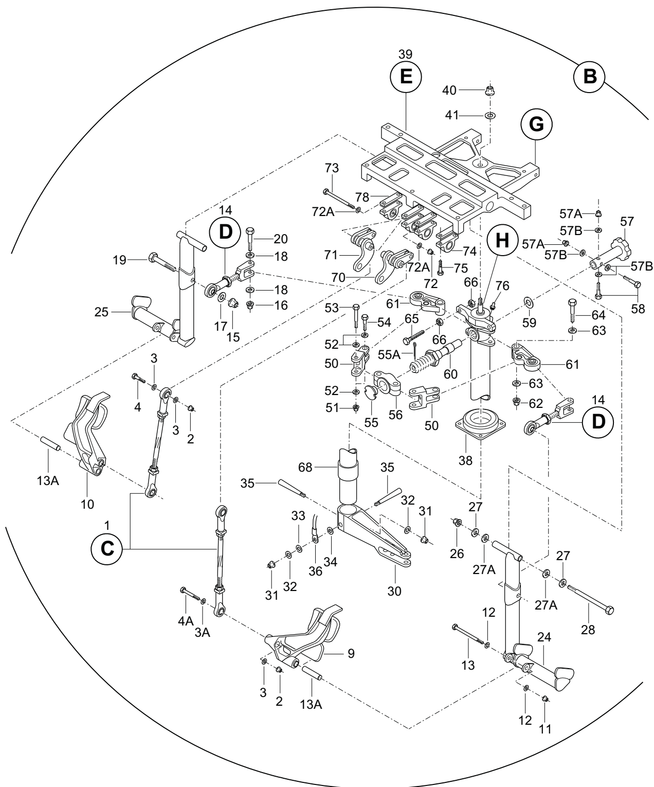
FIGURA 01. CONJUNTO DO PEDAL INST (FOLHA 2 DE 3) FIGURE 01. PEDALS INST (SHEET 2 OF 3)
