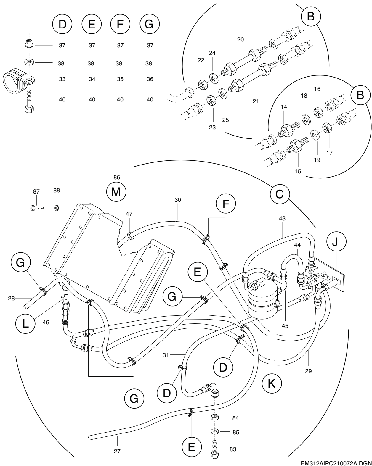
FIGURA 03. SISTEMA FREON INSTL (FOLHA 2 DE 5) FIGURE 03. FREON-CYCLE AIR CONDITIONING SYSTEM INSTL (SHEET 2 OF 5)
