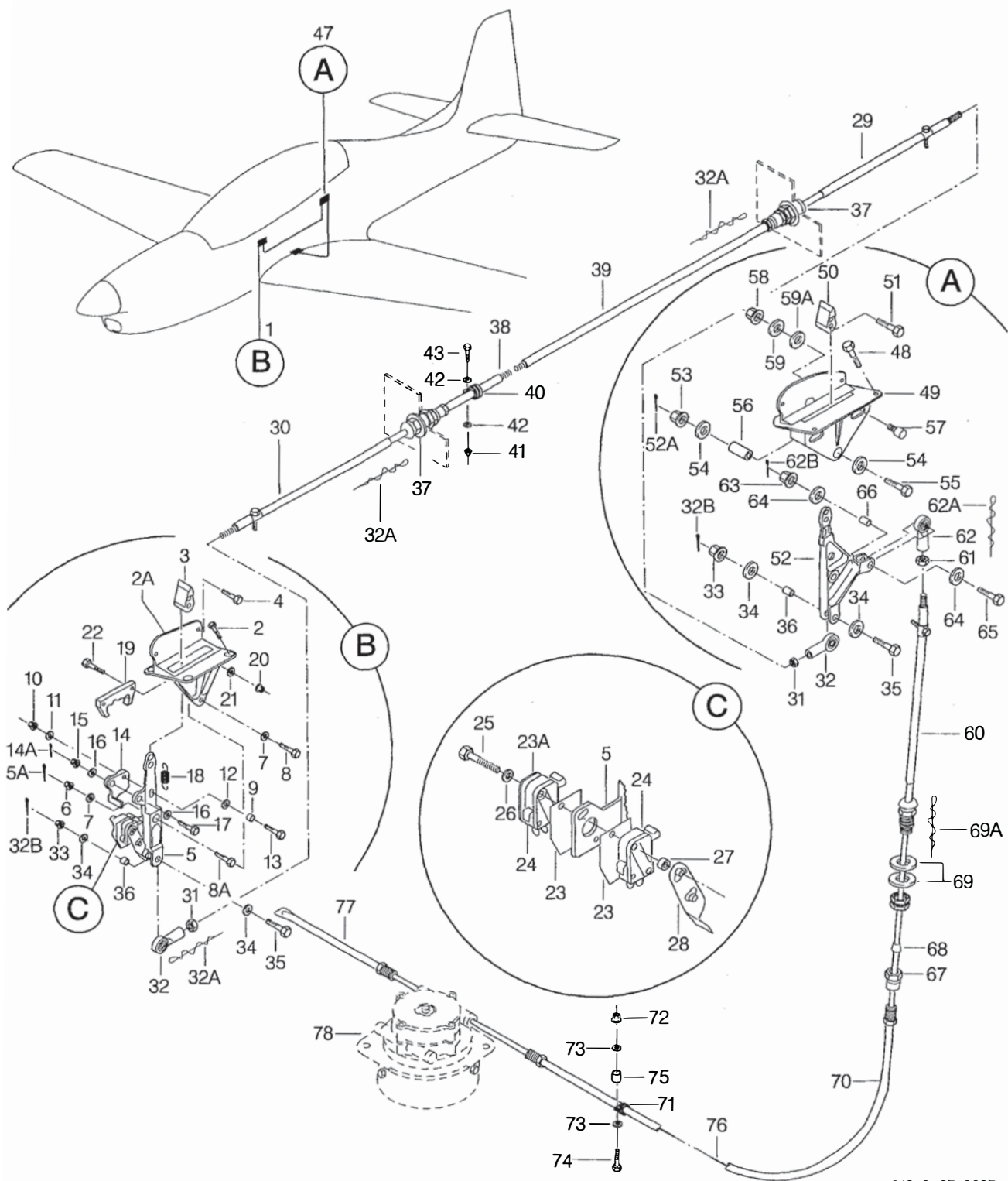
FIGURA 02. SISTEMA DE COMANDO INSTL, FLAPES FIGURE 02. CONTROL SYSTEM INSTL, FLAP
