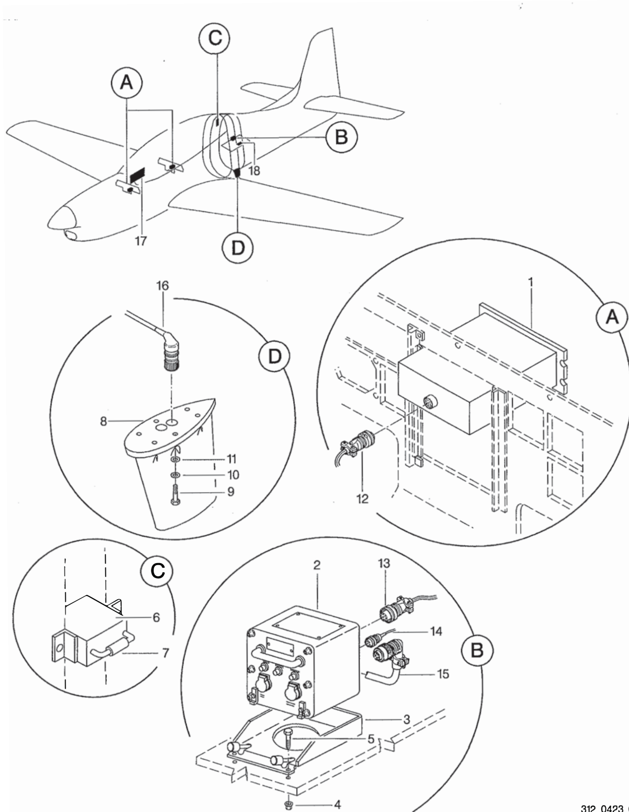
FIGURA 01. SISTEMA UHF INSTL FIGURE 01. UHF SYSTEM INSTL
