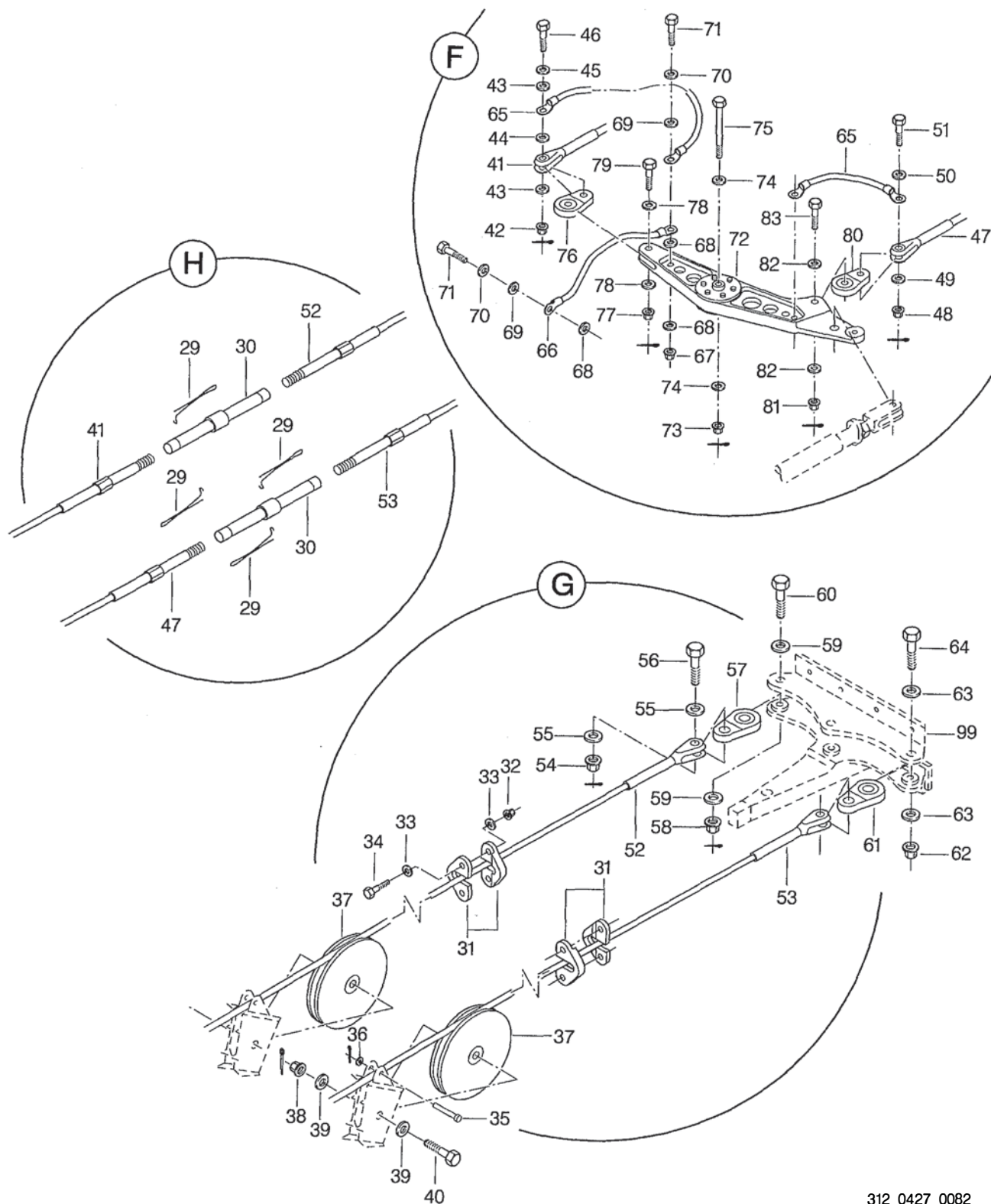
FIGURA 01. COMANDO DO LEME INSTL (FOLHA 3 DE 3) FIGURE 01. RUDDER CONTROL INSTL (SHEET 3 OF 3)
