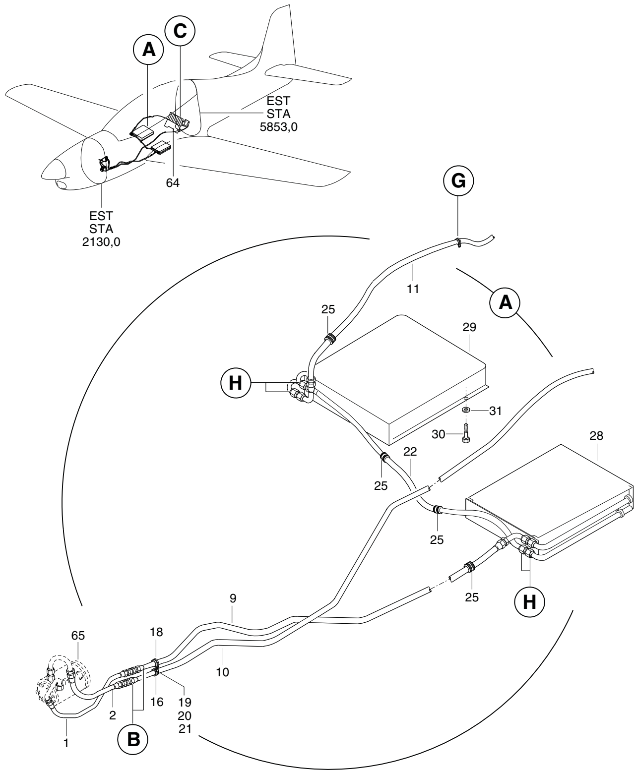
FIGURA 02. SISTEMA FREON INSTL (FOLHA 1 DE 4) FIGURE 02. FREON-CYCLE AIR CONDITIONING SYSTEM INSTL (SHEET 1 OF 4)
