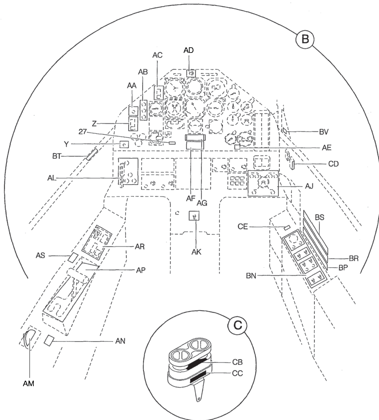
FIGURA 02. INSCRICOES E MARCACOES INTERNAS INSTL (FOLHA 2 DE 13) FIGURE 02. INTERIOR PLACARDS & MARKINGS INSTL (SHEET 2 OF 13)
