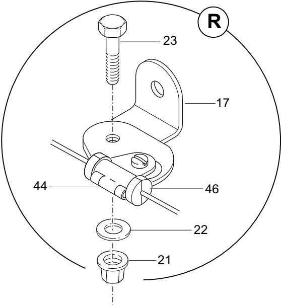
FIGURA 01. SISTEMA DE DETECCAO DE FOGO INSTL, MOTOR (FOLHA 5 DE 6) FIGURE 01. FIRE DETECTION SYSTEM INSTL, ENGINE (SHEET 5 OF 6)
