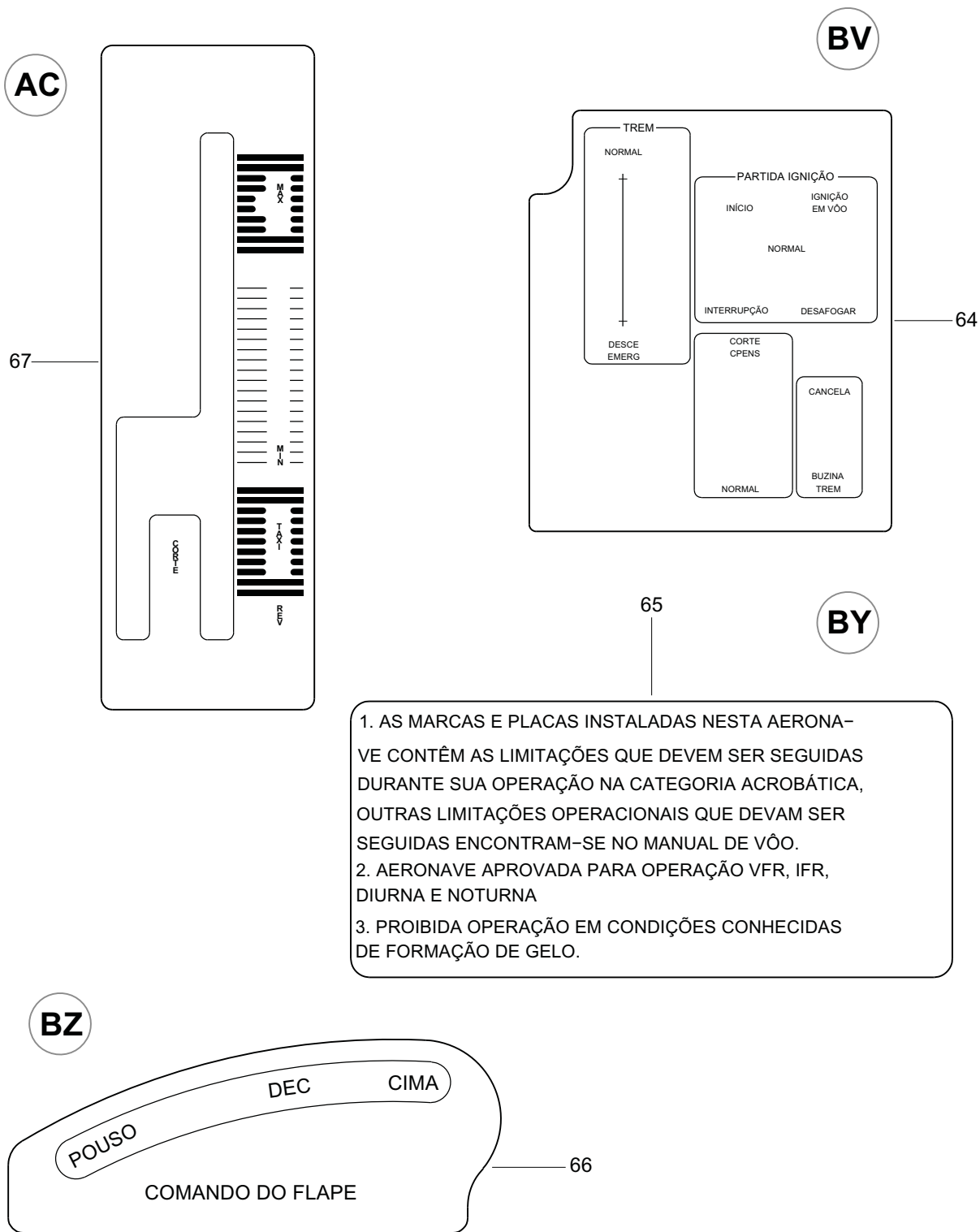
FIGURA 01. INSCRICOES E MARCACOES INTERNAS INSTL (FOLHA 14 DE 15) FIGURE 01. INTERIOR PLACARDS & MARKINGS INSTL (SHEET 14 OF 15)
