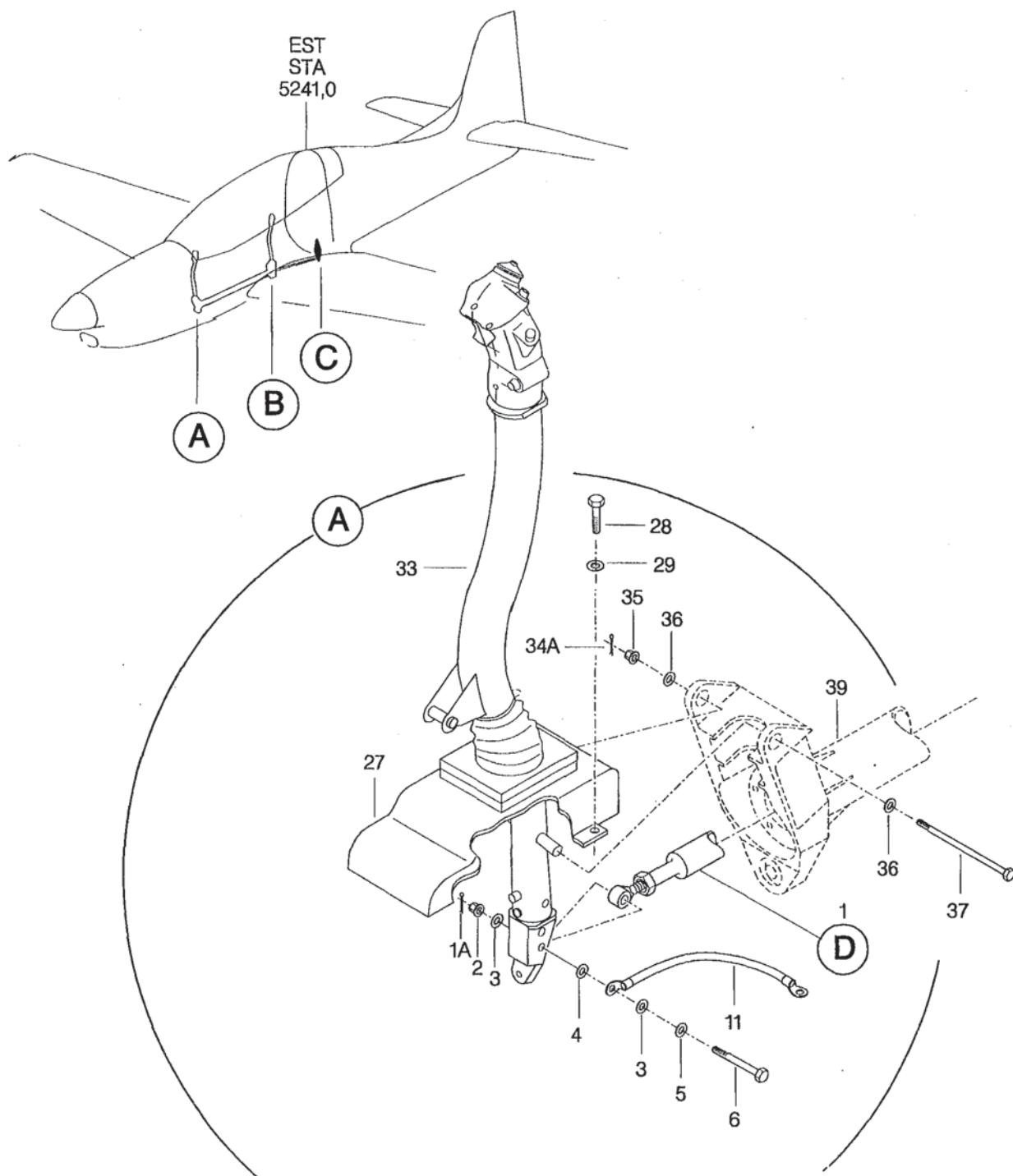
FIGURA 01. COMANDO DO PROFUNDOR INSTL, FUSELAGEM DIANTEIRA (FOLHA 1 DE 3) FIGURE 01. ELEVATOR CONTROL INSTL, FUSELAGE FWD SECTION (SHEET 1 OF 3)
