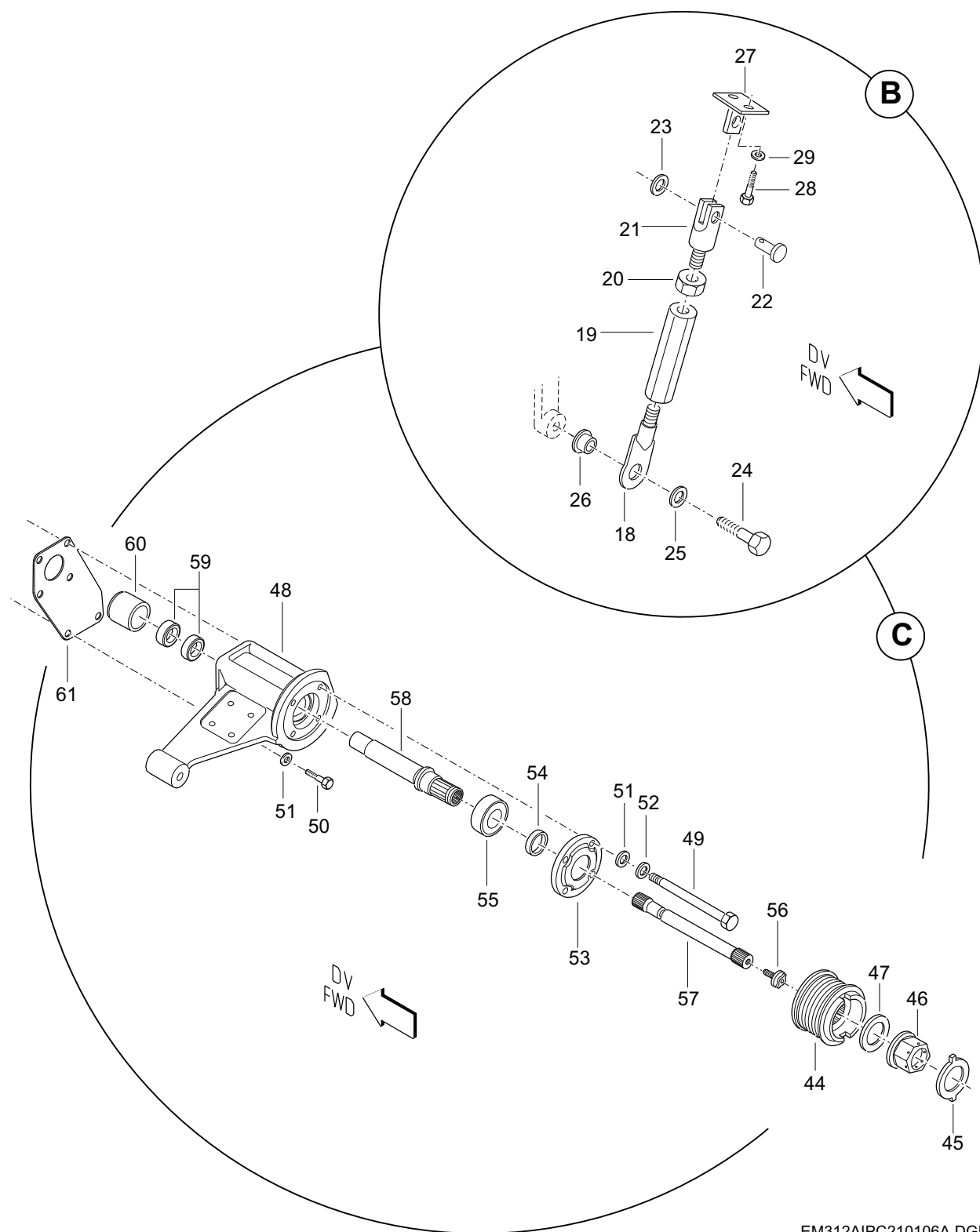
FIGURA 07. INSTALACAO DO COMPRESSOR (FOLHA 1 DE 2) FIGURE 07. COMPRESSOR INSTL (SHEET 1 OF 2)
