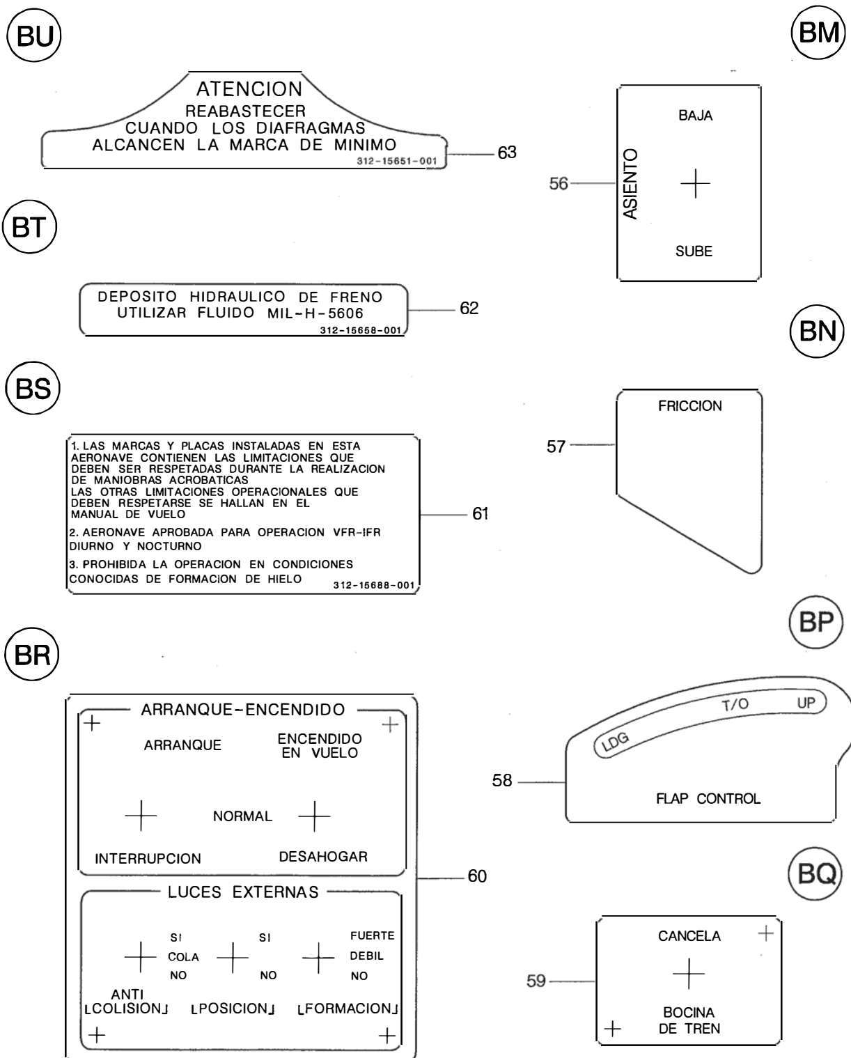
FIGURA 05. INSCRICOES E MARCACOES INTERNAS INSTL (FOLHA 10 DE 12) FIGURE 05. INTERIOR PLACARDS & MARKINGS INSTL (SHEET 10 OF 12)
