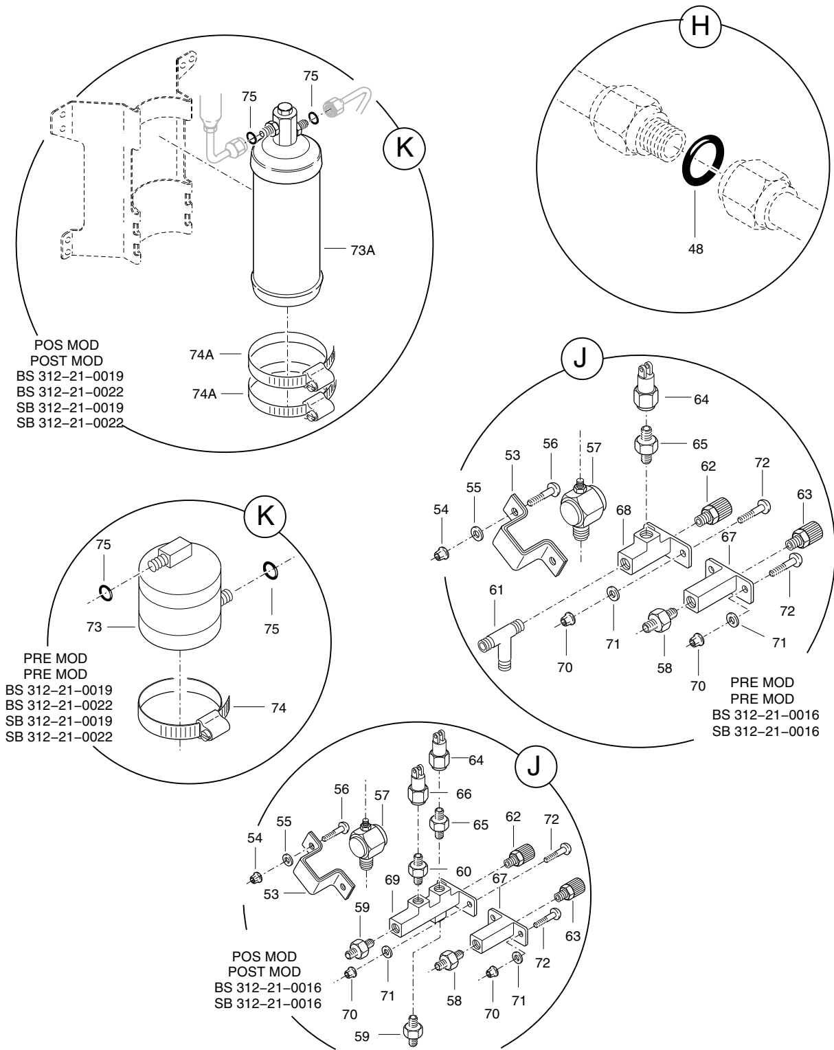
FIGURA 03. SISTEMA FREON INSTL (FOLHA 3 DE 5) FIGURE 03. FREON-CYCLE AIR CONDITIONING SYSTEM INSTL (SHEET 3 OF 5)
