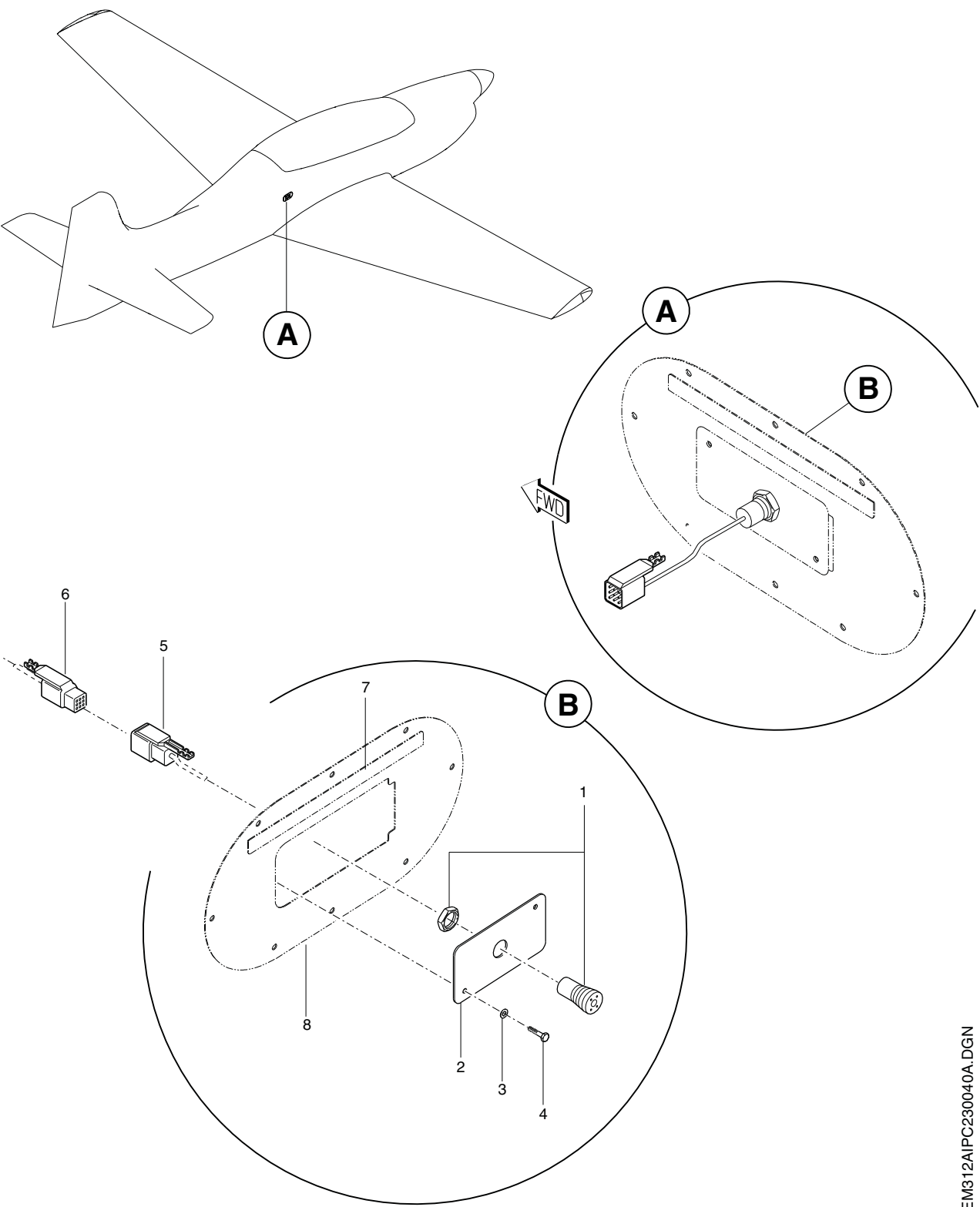
FIGURA 01. AUDIO RAMPA INSTAL FIGURE 01. AUDIO RAMP INSTALLATION
