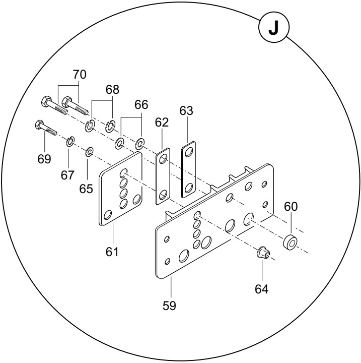
FIGURA 01. BATERIA E ACESSORIOS INSTL (FOLHA 4 DE 4) FIGURE 01. BATTERY & ACESSORIES INSTL (SHEET 4 OF 4)
