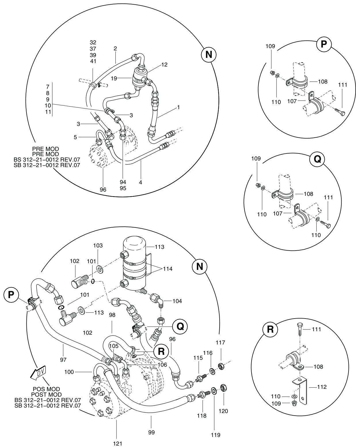
FIGURA 03. SISTEMA FREON INSTL (FOLHA 5 DE 5) FIGURE 03. FREON-CYCLE AIR CONDITIONING SYSTEM INSTL (SHEET 5 OF 5)
