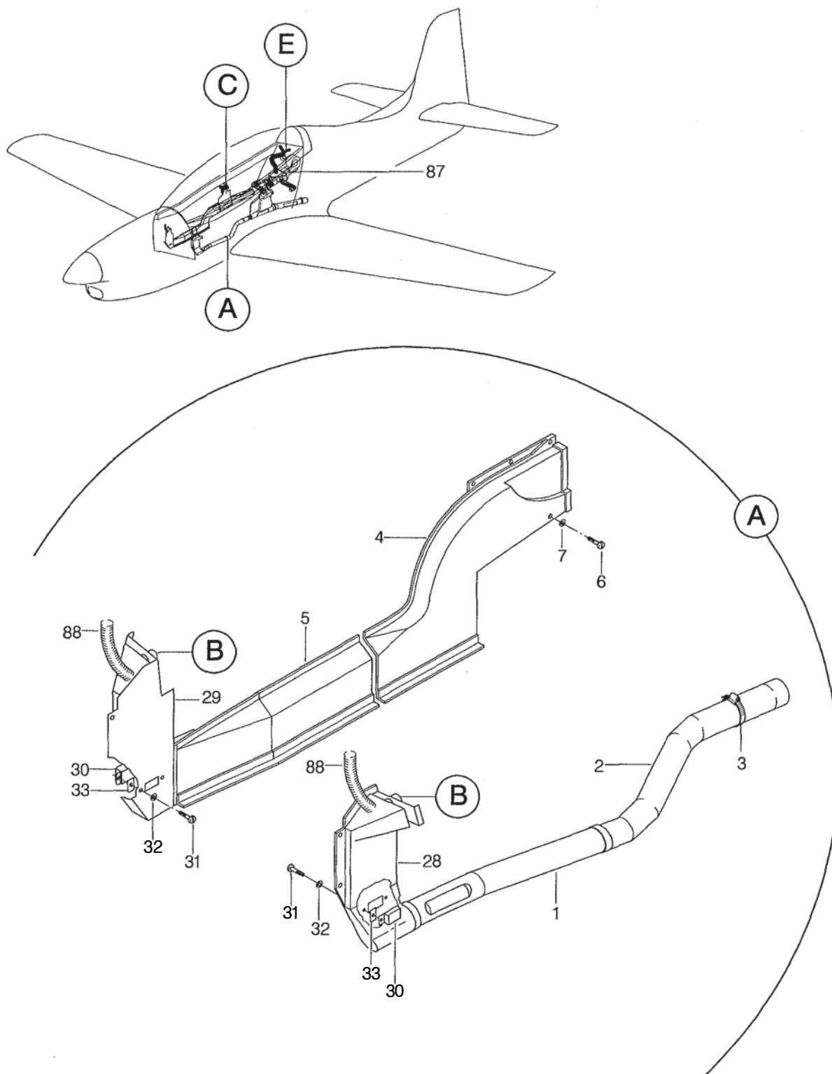
FIGURA 04. DISTRIBUICAO DE AR CONDICIONADO INSTL (FOLHA 1 DE 3) FIGURE 04. AIR CONDITIONING DISTRIBUTION INSTL (SHEET 1 OF 3)
