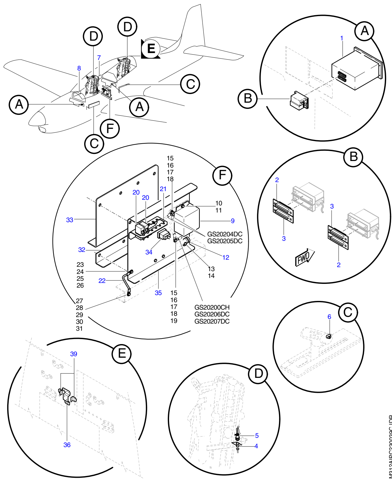
FIGURA 02. SISTEMA DE AUDIO INSTL FIGURE 02. AUDIO SYSTEM INSTL
