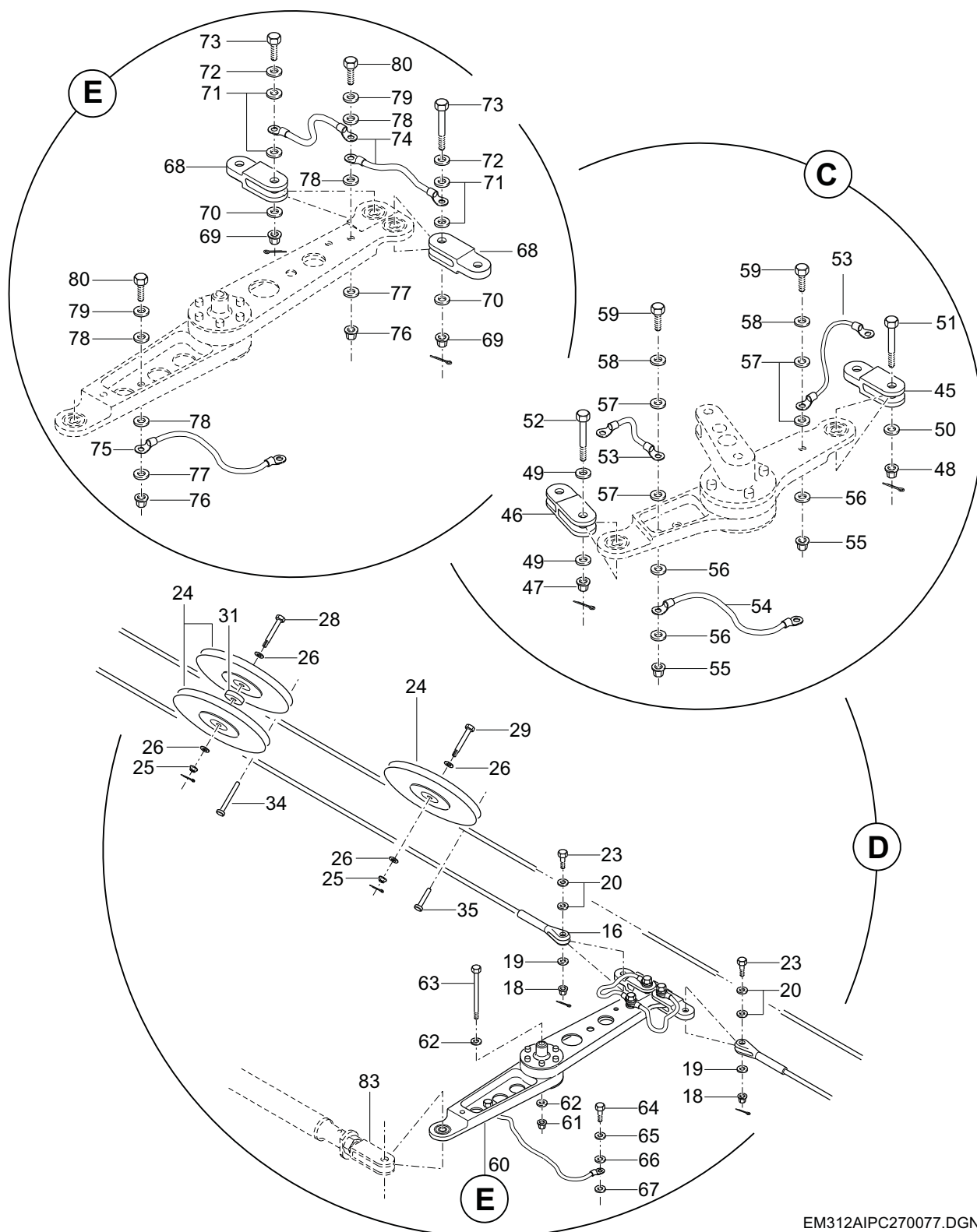
FIGURA 02. COMANDO DO AILERON (FOLHA 2 DE 2) FIGURE 02. AILERON CONTROL INST, WINGS (SHEET 2 OF 2)
