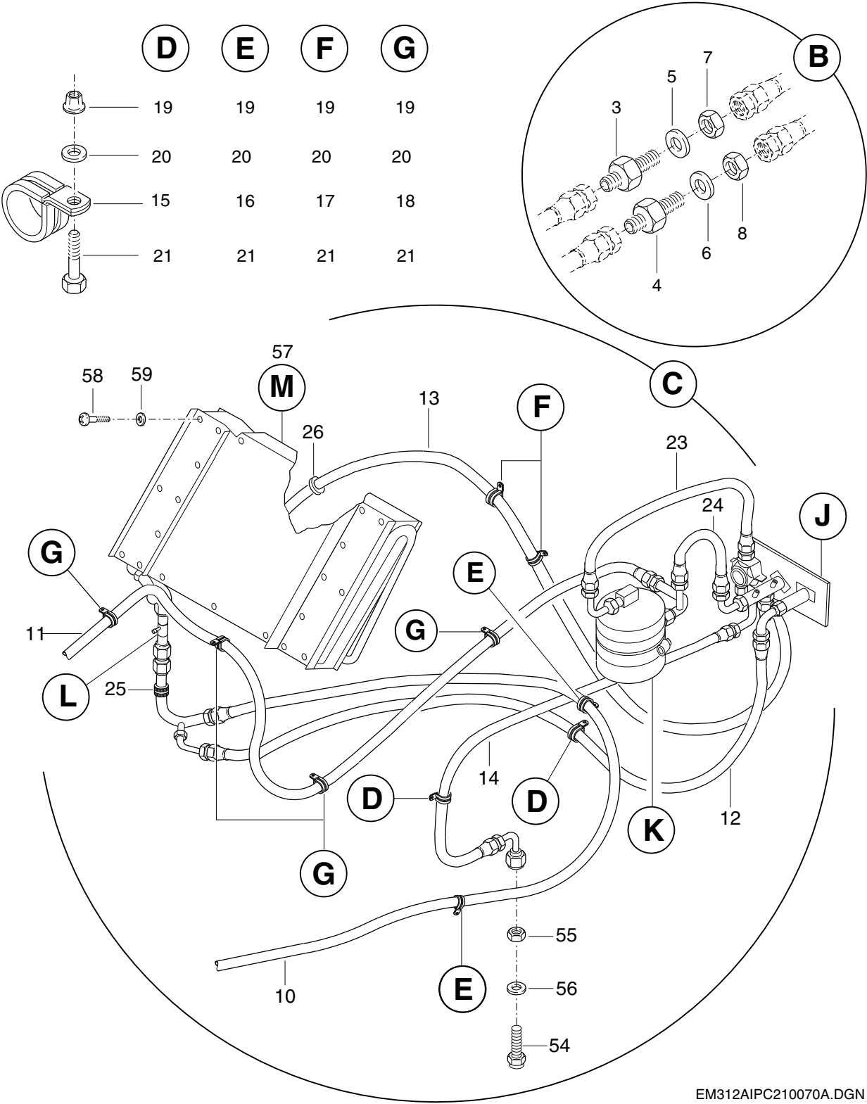
FIGURA 02. SISTEMA FREON INSTL (FOLHA 2 DE 4) FIGURE 02. FREON-CYCLE AIR CONDITIONING SYSTEM INSTL (SHEET 2 OF 4)
