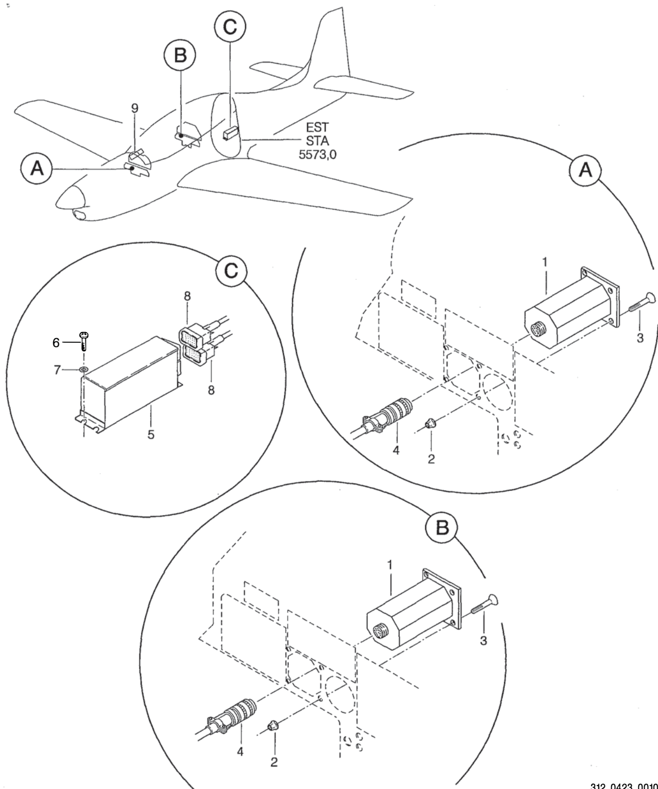
FIGURA 01. SISTEMA DE TRANSFERENCIA DE RADIO INSTL FIGURE 01. RADIO CONTROL TRANSFER SYSTEM INSTL
