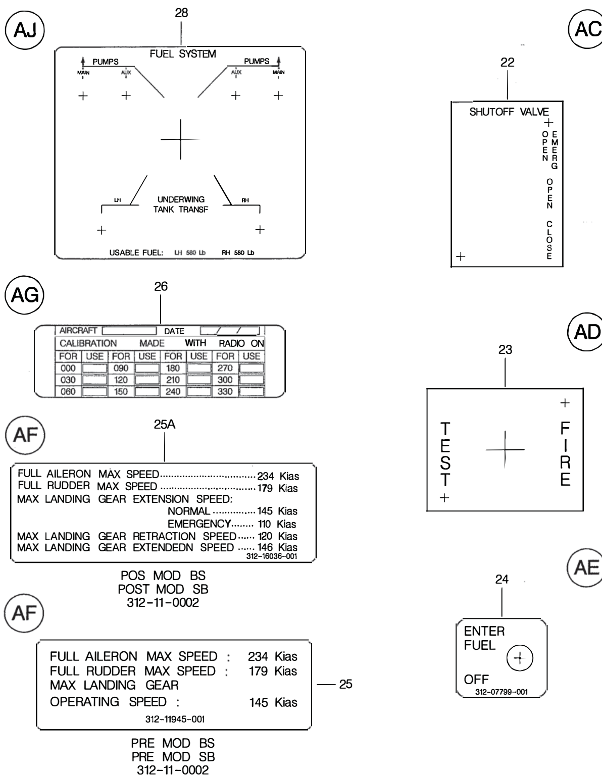
FIGURA 02. INSCRICOES E MARCACOES INTERNAS INSTL (FOLHA 6 DE 13) FIGURE 02. INTERIOR PLACARDS & MARKINGS INSTL (SHEET 6 OF 13)
