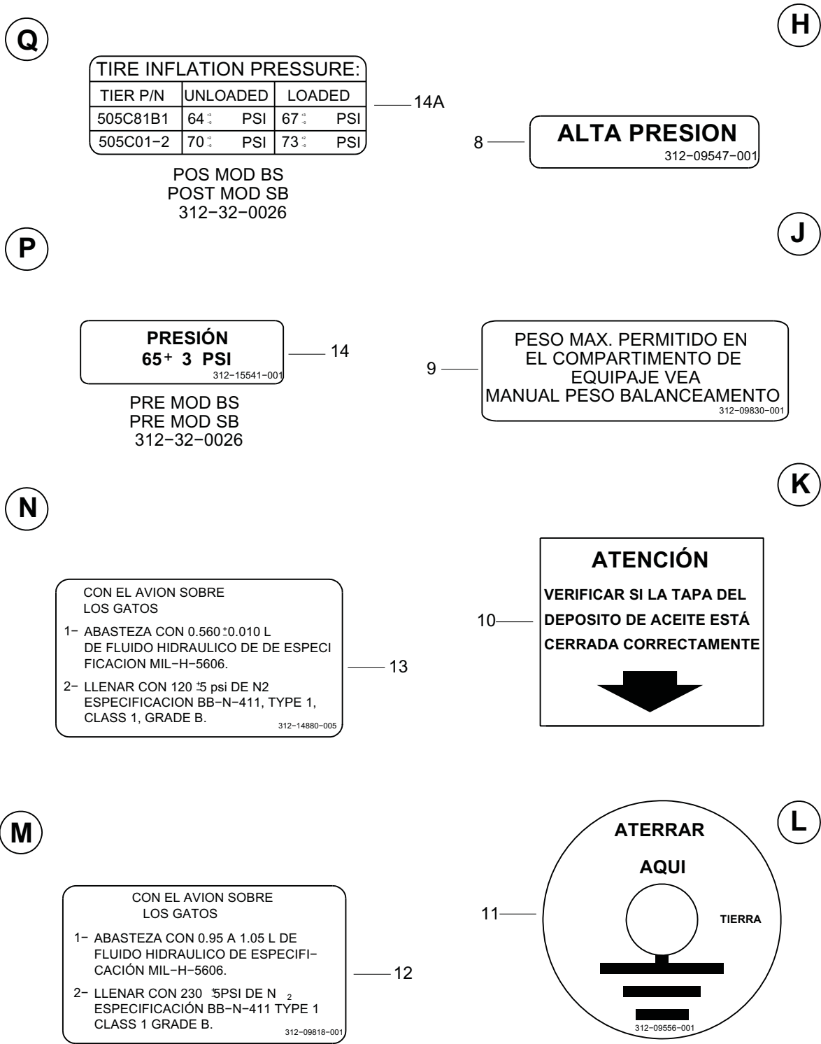
FIGURA 06. INSCRICOES E MARCACOES EXTERNAS INSTL (FOLHA 4 DE 6) FIGURE 06. EXTERIOR PLACARDS & MARKINGS INSTL (SHEET 4 OF 6)
