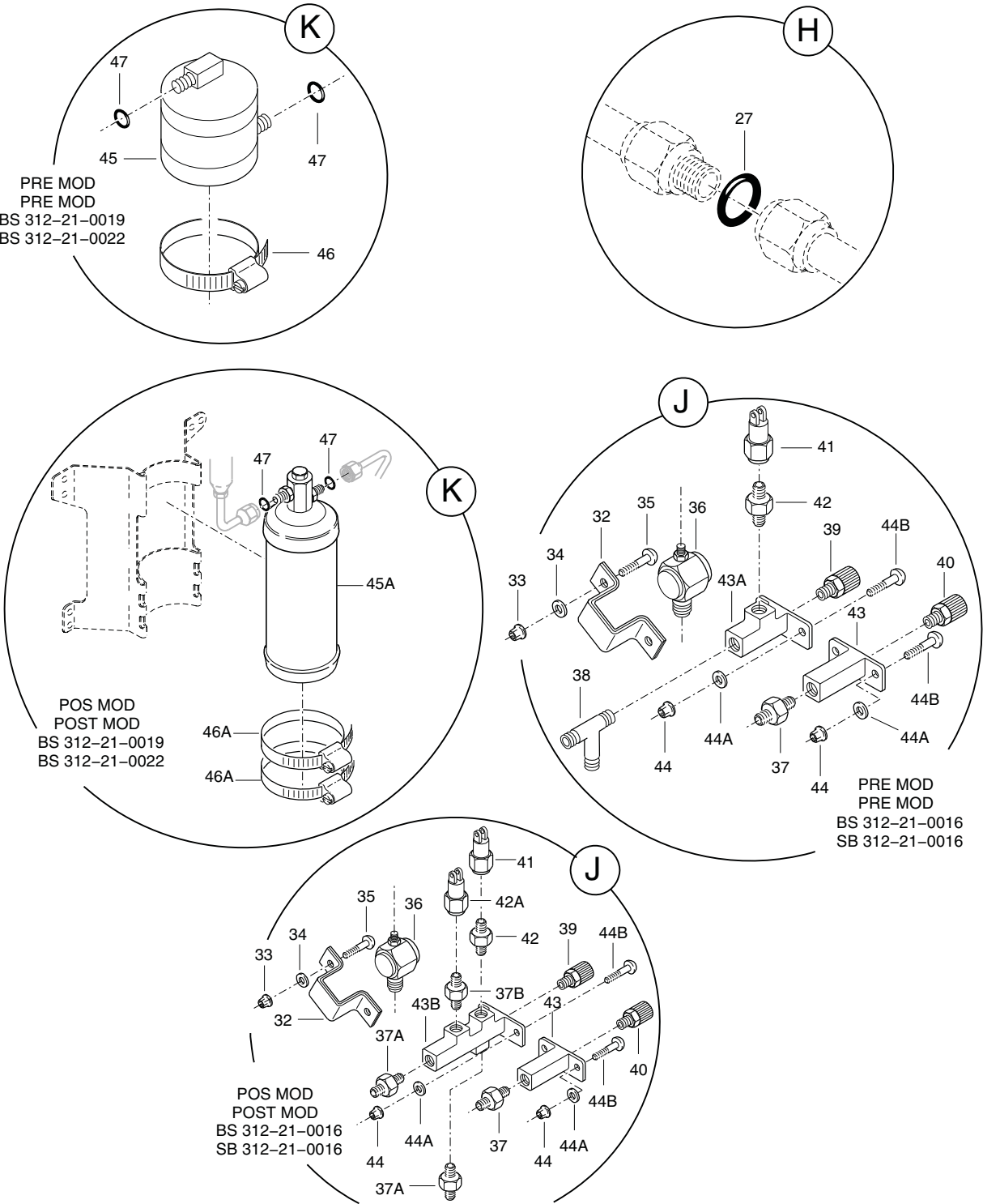
FIGURA 02. SISTEMA FREON INSTL (FOLHA 3 DE 4) FIGURE 02. FREON-CYCLE AIR CONDITIONING SYSTEM INSTL (SHEET 3 OF 4)
