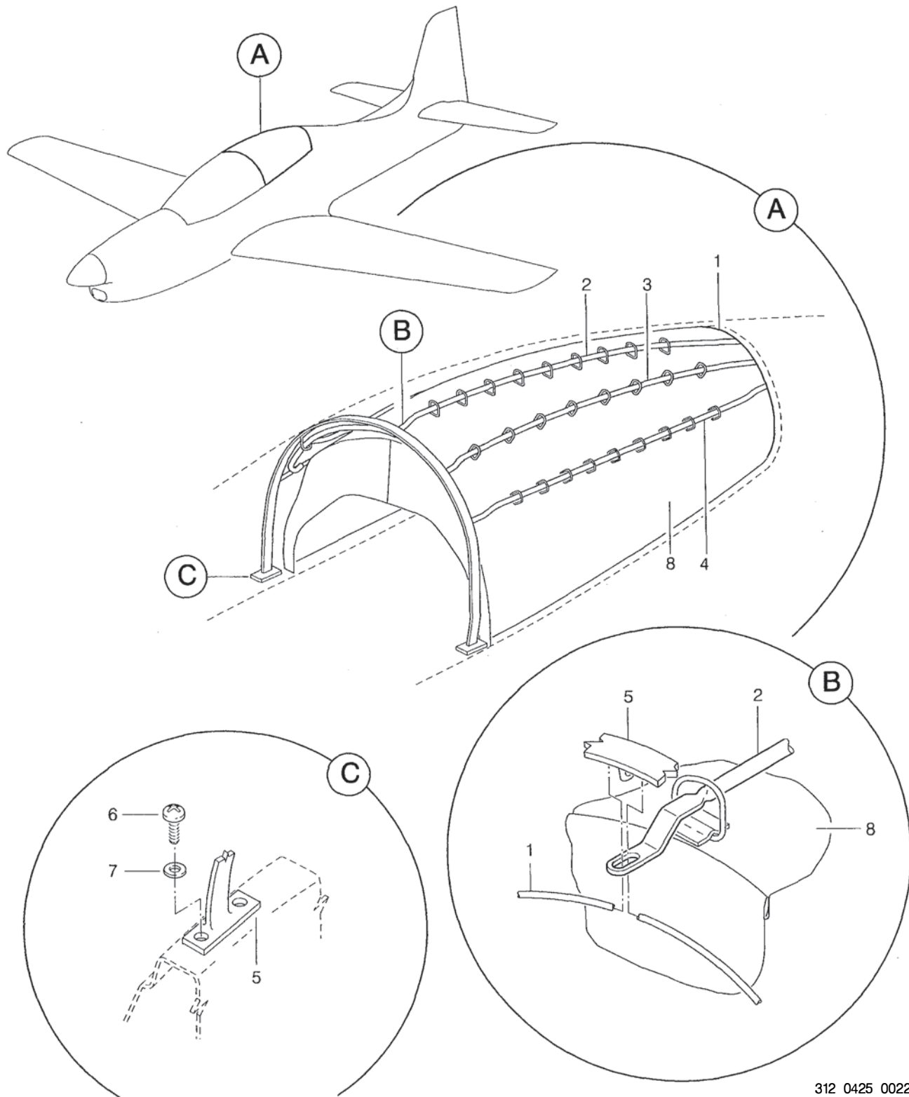
FIGURA 05. CAPOTA PI/VOO POR INSTRUMENTO INSTL FIGURE 05. BLIND INSTRUMENT FLYING HOOD INSTL
