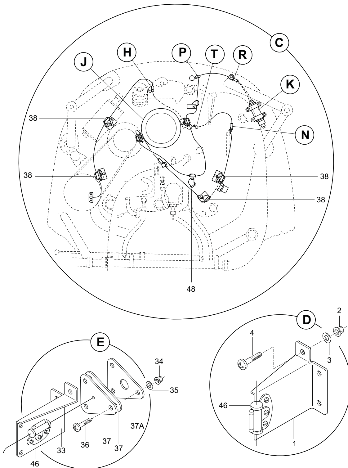
FIGURA 01. SISTEMA DE DETECCAO DE FOGO INSTL, MOTOR (FOLHA 2 DE 6) FIGURE 01. FIRE DETECTION SYSTEM INSTL, ENGINE (SHEET 2 OF 6)
