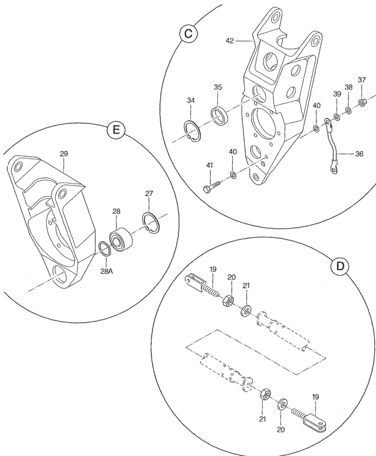
FIGURA 01. COMANDO DO AILERON INSTL, FUSELAGEM (FOLHA 2 DE 2) FIGURE 01. AILERON CONTROL INSTL, FUSELAGE (SHEET 2 OF 2)
