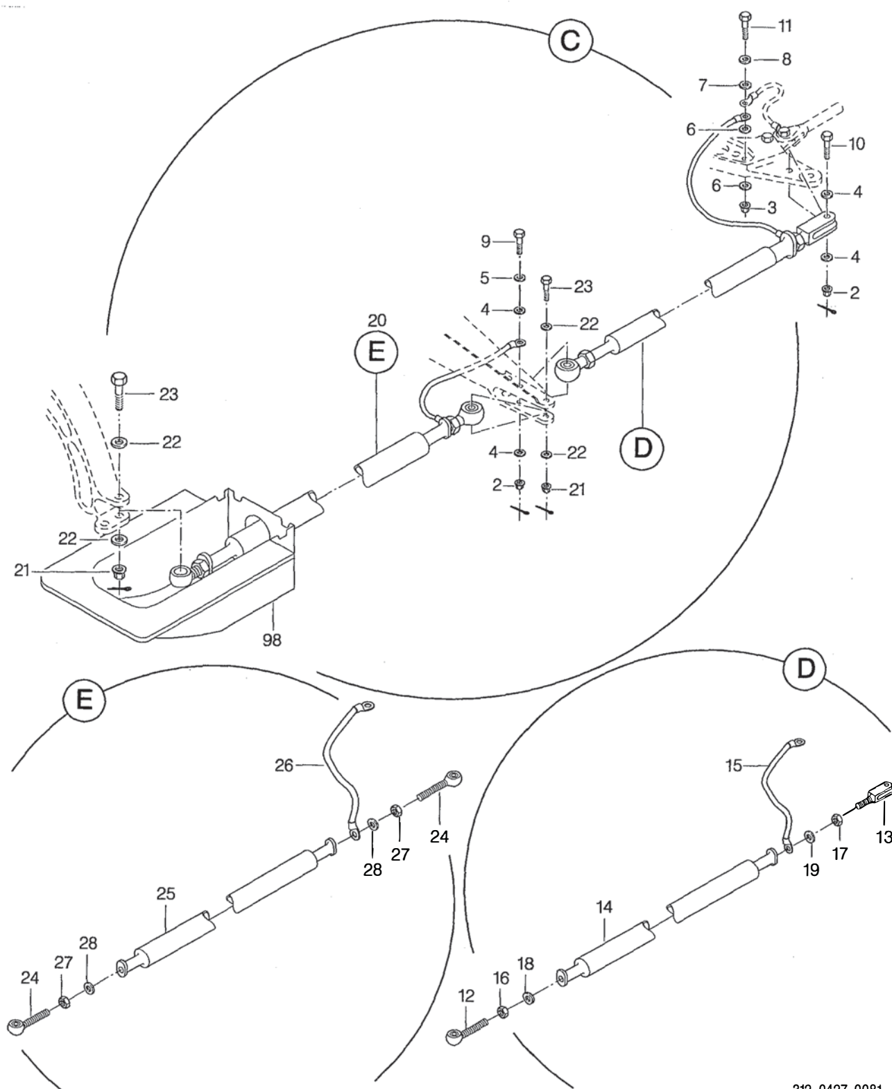
FIGURA 01. COMANDO DO LEME INSTL (FOLHA 2 DE 3) FIGURE 01. RUDDER CONTROL INSTL (SHEET 2 OF 3)
