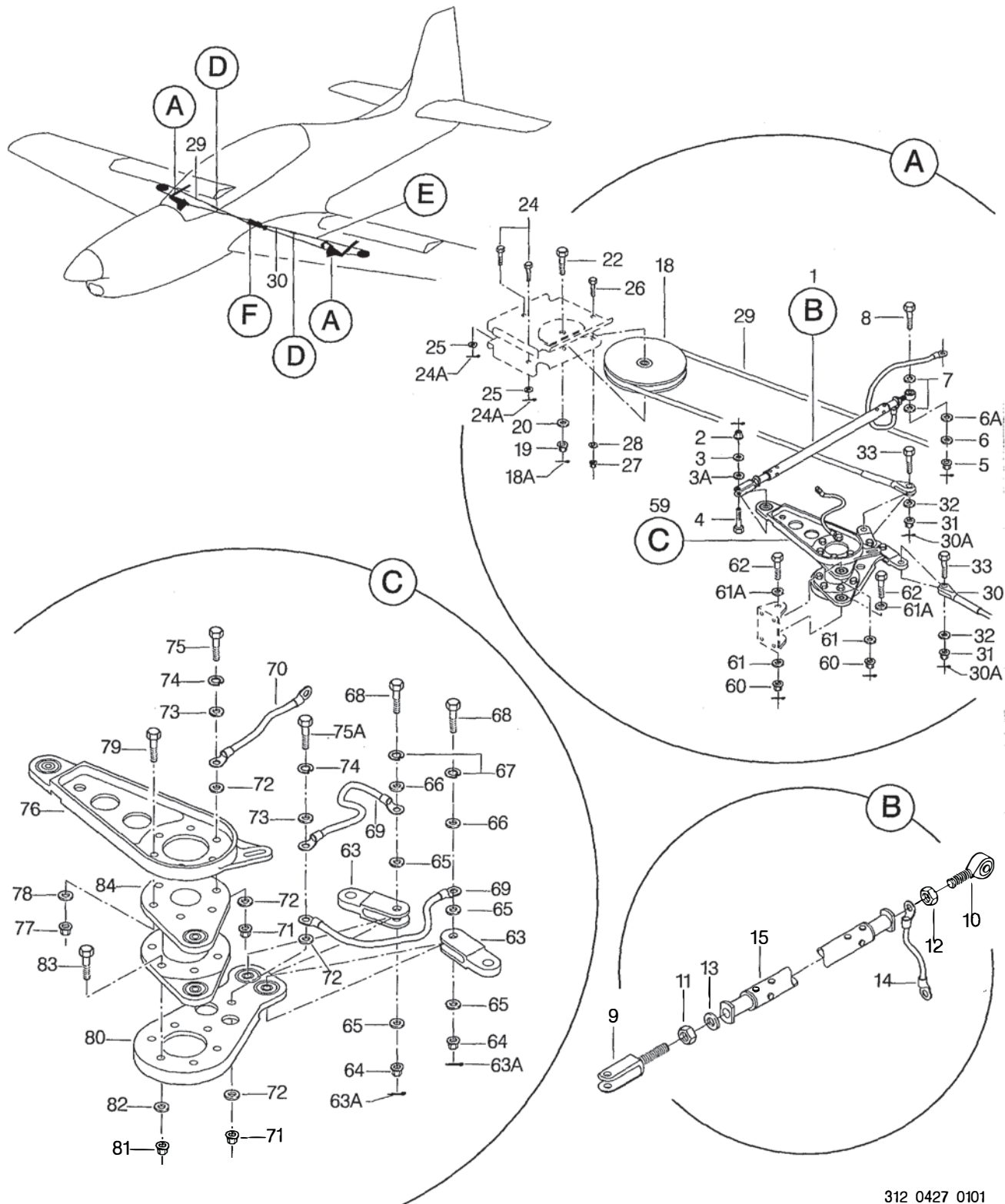
FIGURA 01. INTERLIGACAO DOS FLAPES INSTL (FOLHA 1 DE 2) FIGURE 01. FLAPS INTERCONNECTION INSTL (SHEET 1 OF 2)
