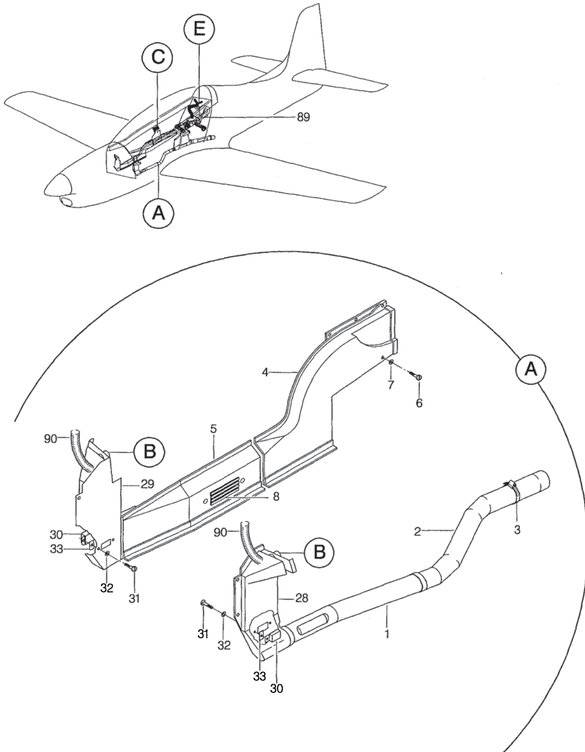
FIGURA 03. DISTRIBUICAO DE AR CONDICIONADO INSTL (FOLHA 1 DE 3) FIGURE 03. AIR CONDITIONING DISTRIBUTION INSTL (SHEET 1 OF 3)
