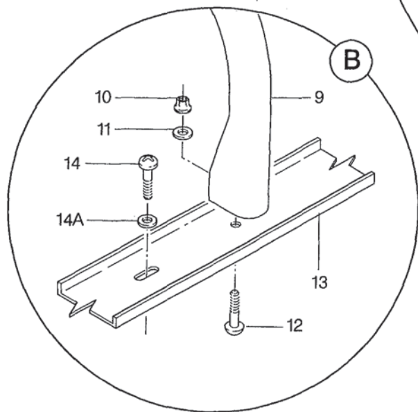
FIGURA 03. CAPOTA P/ VOO POR INSTRUMENTO INSTL FIGURE 03. BLIND INSTRUMENT FLYING HOOD INSTL
