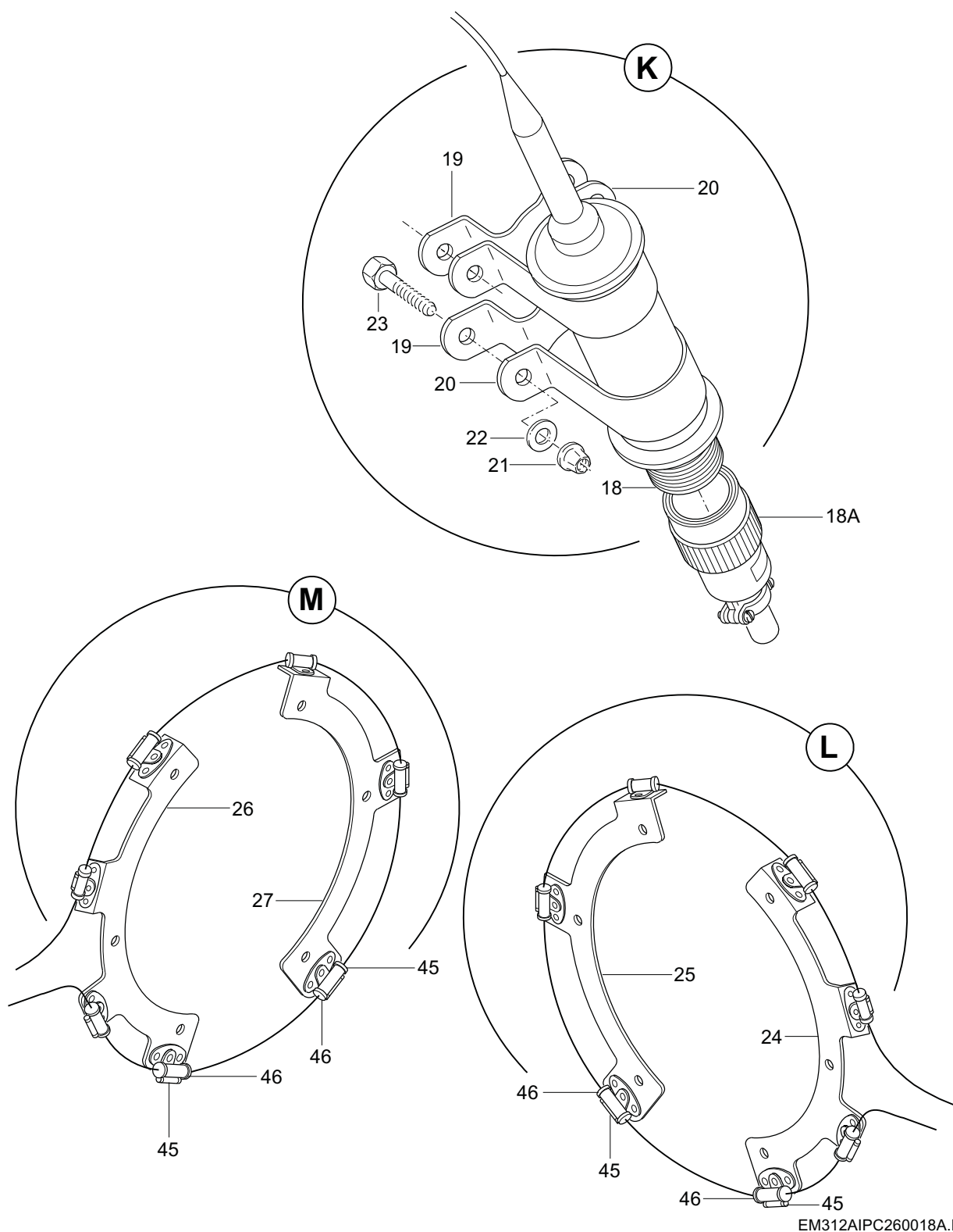
FIGURA 01. SISTEMA DE DETECCAO DE FOGO INSTL, MOTOR (FOLHA 4 DE 6) FIGURE 01. FIRE DETECTION SYSTEM INSTL, ENGINE (SHEET 4 OF 6)
