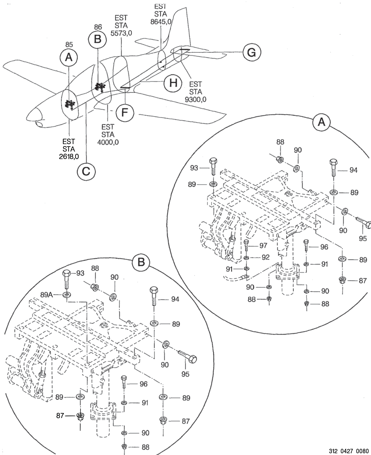
FIGURA 01. COMANDO DO LEME INSTL (FOLHA 1 DE 3) FIGURE 01. RUDDER CONTROL INSTL (SHEET 1 OF 3)
