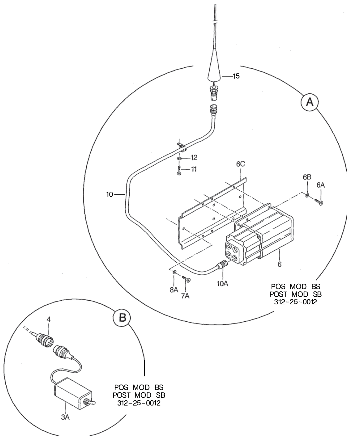
FIGURA 01. TRANSMISSOR DE EMERGENCIA INSTL (FOLHA 2 DE 2) FIGURE 01. EMERGENCY LOCATOR TRANSMITTER INSTL (SHEET 2 OF 2)
