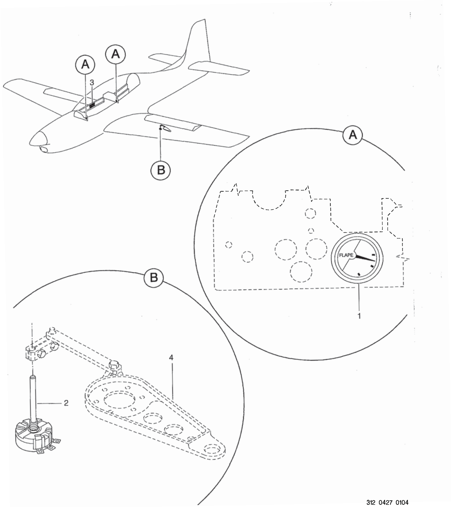
FIGURA 02. INDICACAO DE POSICAO INSTL, FLAPES FIGURE 02. POSITION INDICATING INSTL, FLAP
