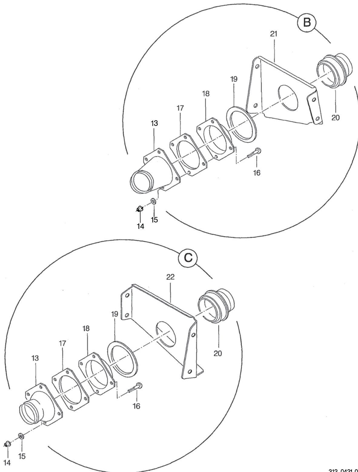
FIGURA 07. DISTRIBUICAO DE AR CONDICIONADO INSTL, POSTO TRASEIRO, EST 4000 A EST 4964 (FOLHA 2 DE 2) FIGURE 07. AIR CONDITIONING DISTRIBUTION INSTL, REAR FLIGHT STATION, STA 4000 THRU STA 4964 (SHEET 2 OF 2)
