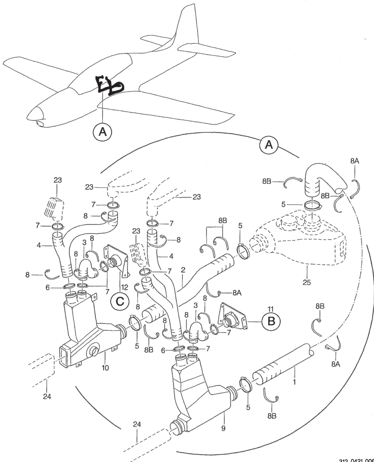
FIGURA 07. DISTRIBUICAO DE AR CONDICIONADO INSTL, POSTO TRASEIRO, EST 4000 A EST 4964 (FOLHA 1 DE 2) FIGURE 07. AIR CONDITIONING DISTRIBUTION INSTL, REAR FLIGHT STATION, STA 4000 THRU STA 4964 (SHEET 1 OF 2)
