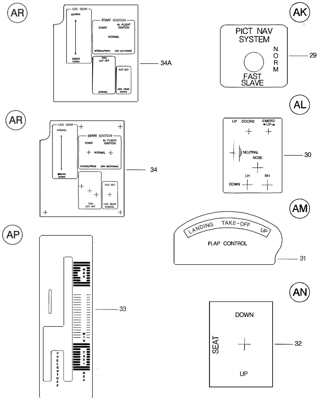
FIGURA 02. INSCRICOES E MARCACOES INTERNAS INSTL (FOLHA 7 DE 13) FIGURE 02. INTERIOR PLACARDS & MARKINGS INSTL (SHEET 7 OF 13)
