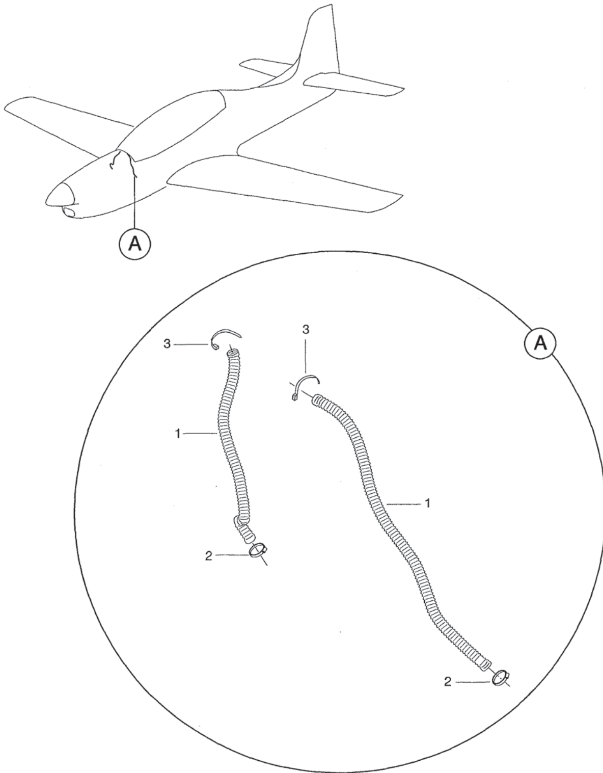
FIGURA 02. VENTILACAO DA CAPOTA INSTL FIGURE 02. CANOPY DEFOGGING INSTL
