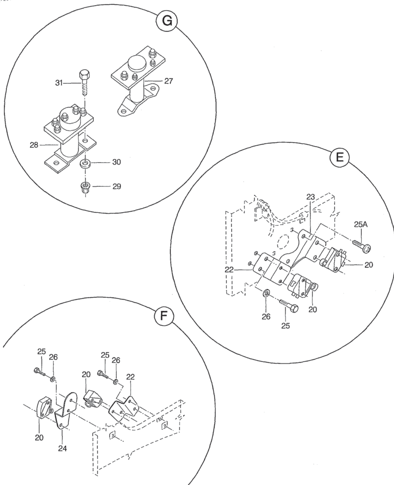
FIGURA 02. CONTROLE DO AR CONDICIONADO INSTL (FOLHA 2 DE 2) FIGURE 02. AIR CONDITIONING CONTROL SYSTEM INSTL (SHEET 2 OF 2)
