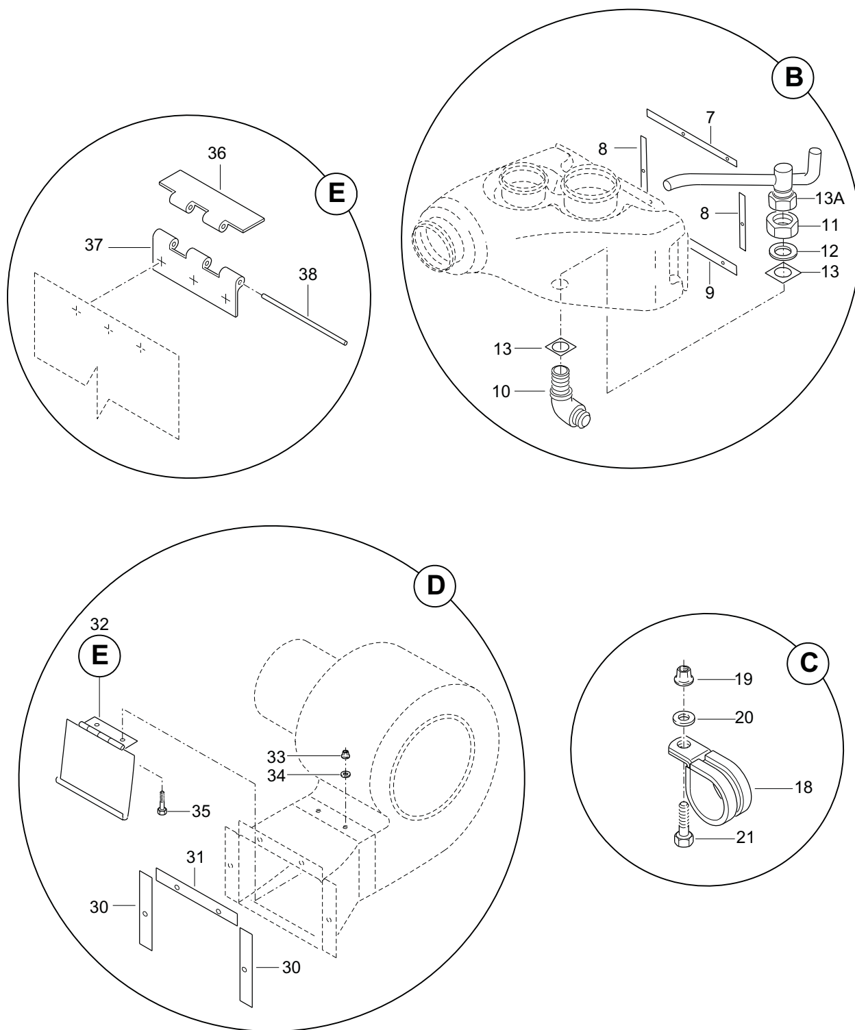
FIGURA 08. DISTRIBUICAO DE AR CONDICIONADO INSTL, POSTO TRASEIRO, EST 4964 A EST 5573 (FOLHA 2 DE 2) FIGURE 08. AIR CONDITIONING DISTRIBUTION INSTL, REAR FLIGHT STA TION, STA 4964 THRU STA 5573 (SHEET 2 OF 2)
