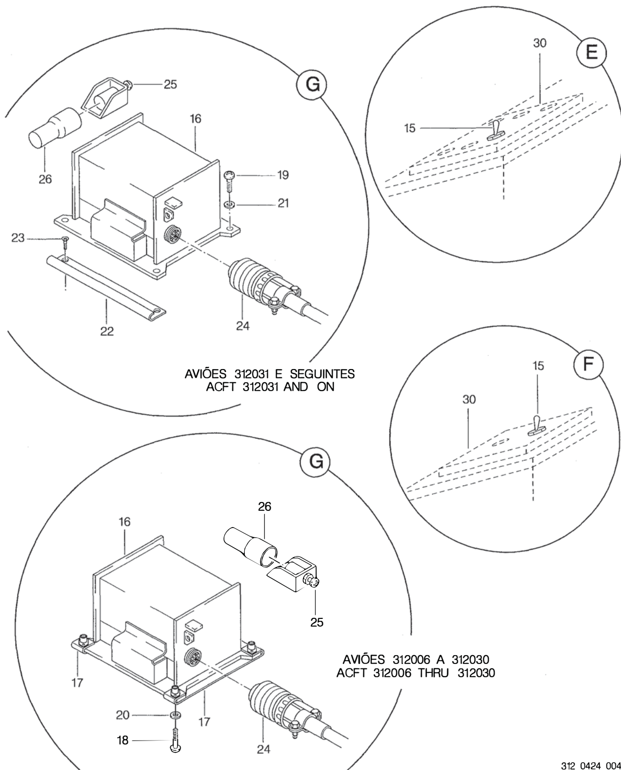
FIGURA 01. SISTEMA DE GERACAO DE CORRENTE CONTINUA INSTL (FOLHA 2 DE 2) FIGURE 01. DIRECT CURRENT GENERATION SYSTEM INSTL (SHEET 2 OF 2)
