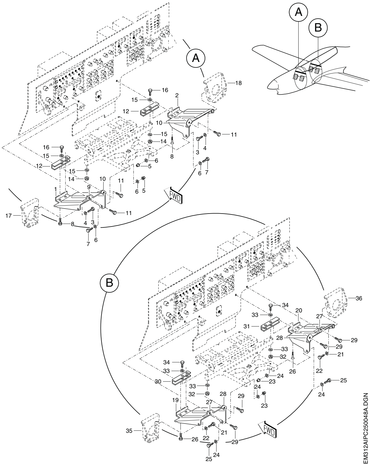
FIGURA 09. KIT CARENAGEM PEDAL, INSTL FIGURE 09. PEDAL FAIRING KIT, INSTL
