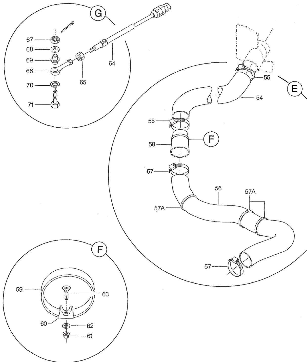
FIGURA 15. VENTILACAO/AQUECIMENTO DA CABINE INSTL (FOLHA 3 DE 3) FIGURE 15. COCKPIT HEATING/VENTILATION SYSTEM INSTL (SHEET 3 OF 3)
