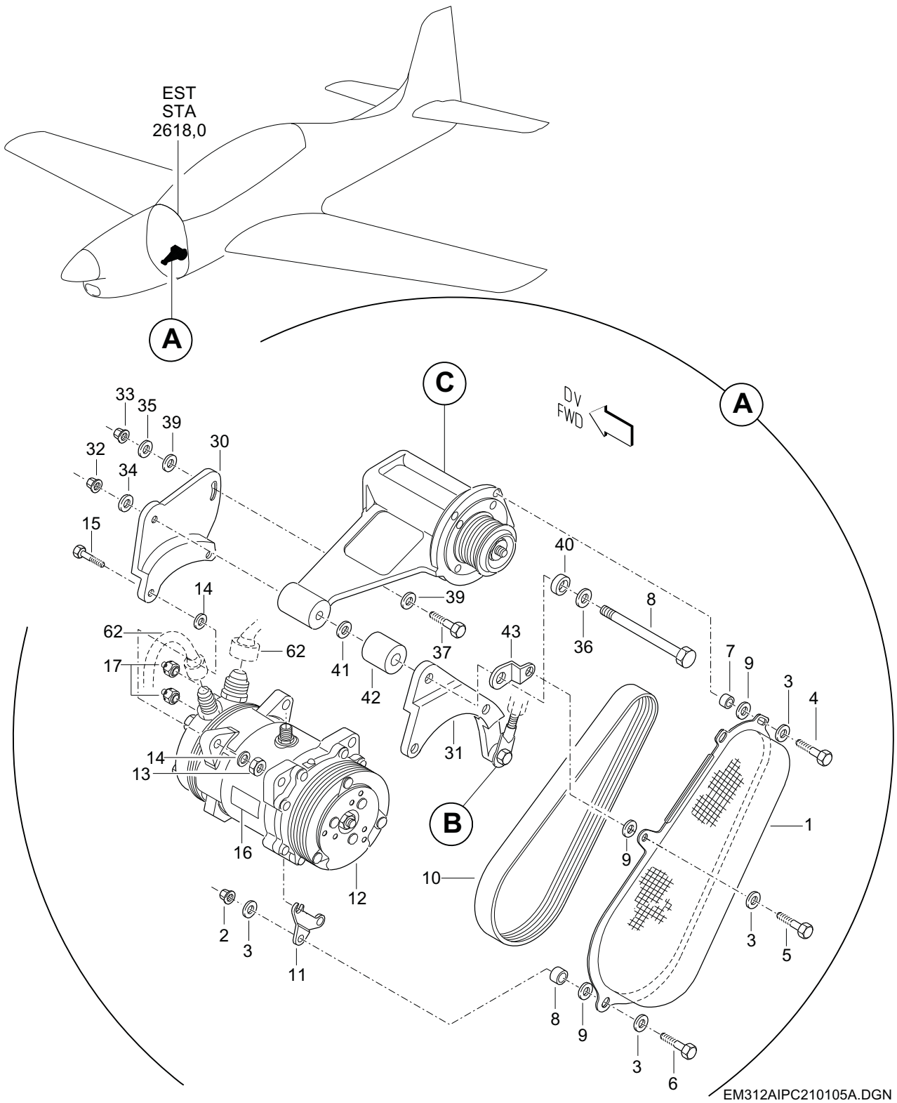
FIGURA 07. INSTALACAO DO COMPRESSOR (FOLHA 1 DE 2) FIGURE 07. COMPRESSOR INSTL (SHEET 1 OF 2)
