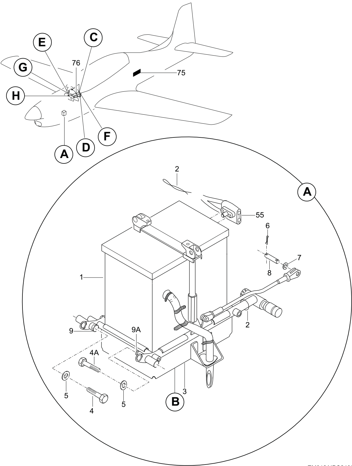
FIGURA 01. BATERIA E ACESSORIOS INSTL (FOLHA 1 DE 4) FIGURE 01. BATTERY & ACESSORIES INSTL (SHEET 1 OF 4)
