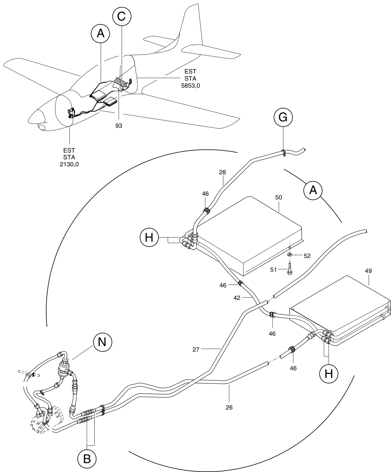
FIGURA 03. SISTEMA FREON INSTL (FOLHA 1 DE 5) FIGURE 03. FREON-CYCLE AIR CONDITIONING SYSTEM INSTL (SHEET 1 OF 5)
