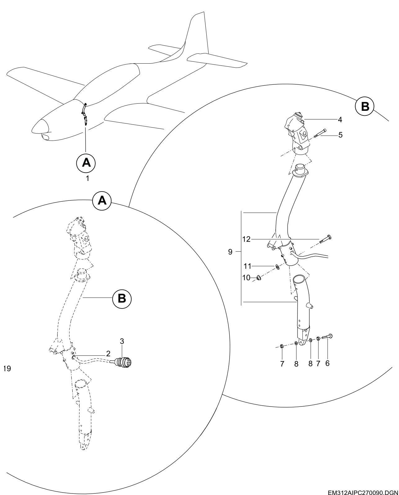
FIGURA 01. CONJUN DOS MANCHES FIGURE 01. CONTROL STICK ASSY
