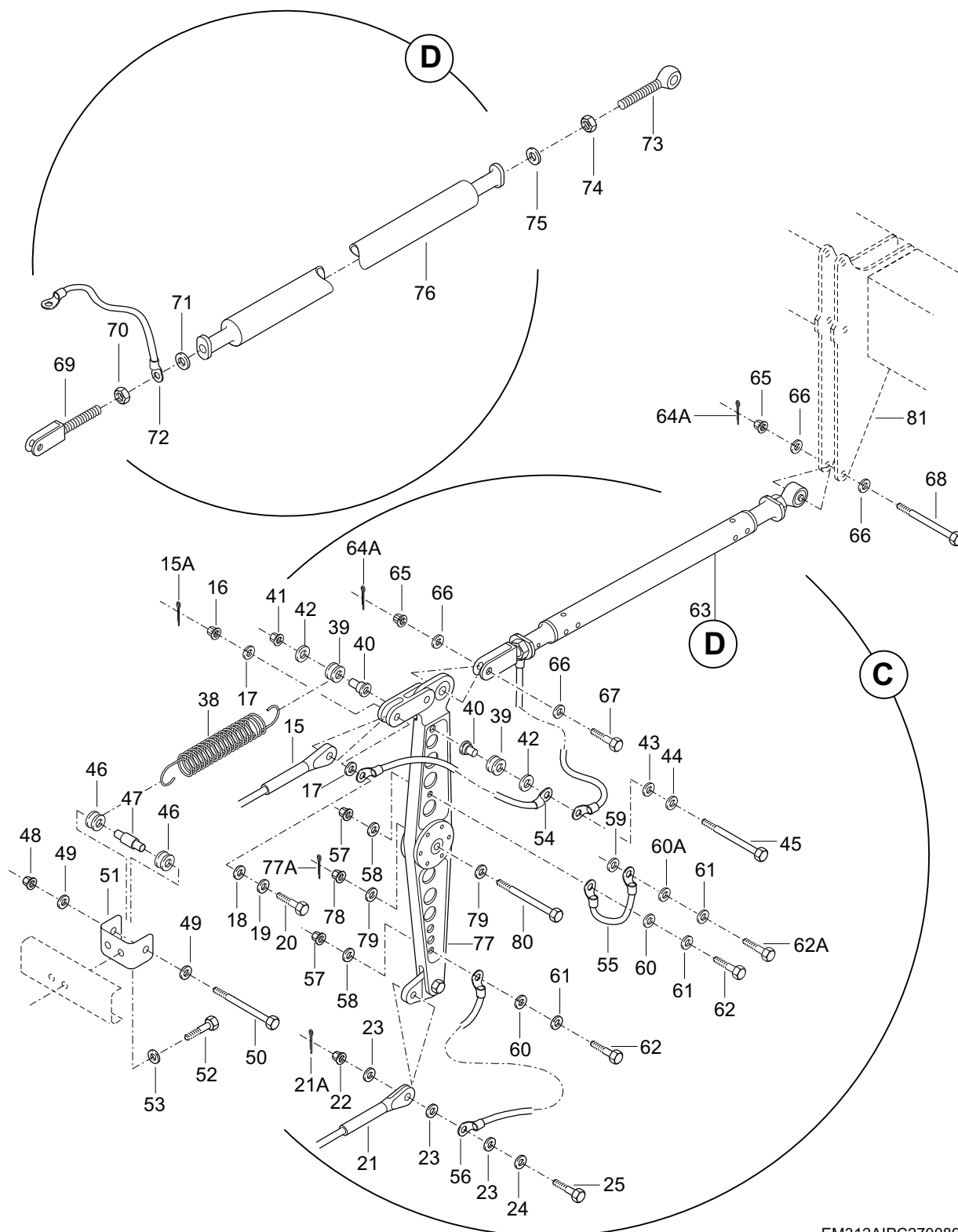
FIGURA 02. COMANDO DO PROFUNDOR INSTL, FUSELAGEM TRASEIRA (FOLHA 2 DE 2) FIGURE 02. ELEVATOR CONTROL INSTL, FUSELAGE AFT SECTION (SHEET 2 OF 2)
