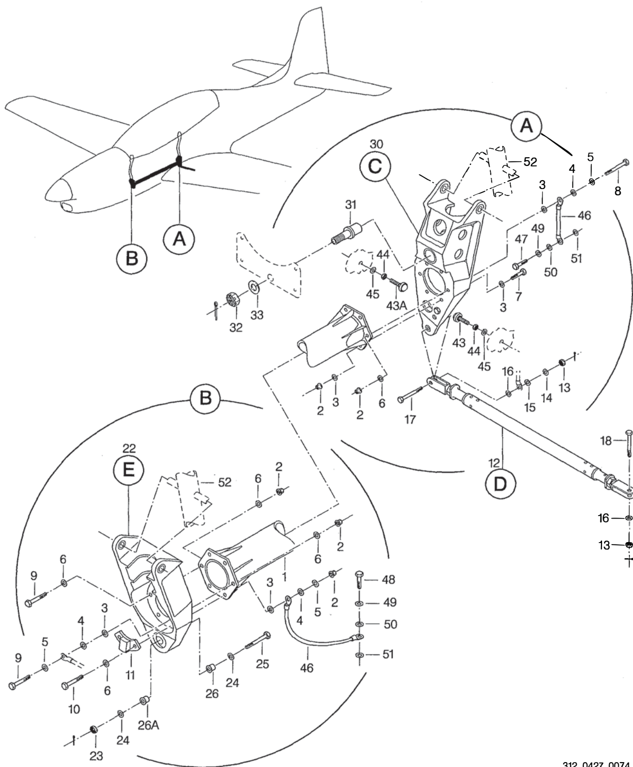
FIGURA 01. COMANDO DO AILERON INSTL, FUSELAGEM (FOLHA 1 DE 2) FIGURE 01. AILERON CONTROL INSTL, FUSELAGE (SHEET 1 OF 2)
