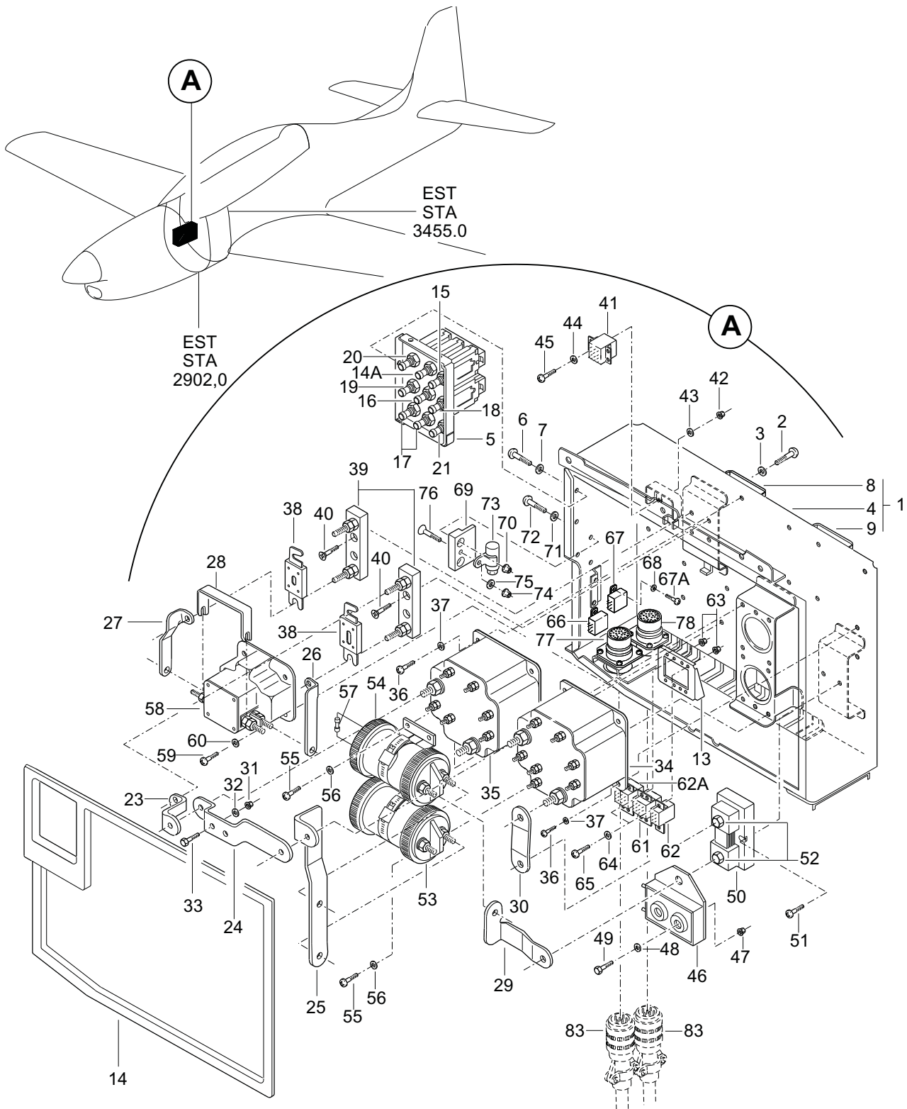
FIGURA 02. CAIXA DE RELES DC INSTL FIGURE 02. DC RELAY BOX INSTL
