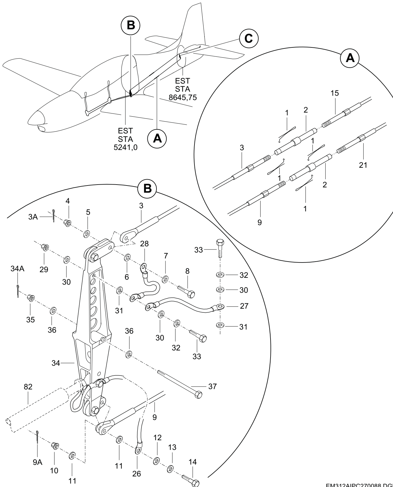
FIGURA 02. COMANDO DO PROFUNDOR INSTL, FUSELAGEM TRASEIRA (FOLHA 1 DE 2) FIGURE 02. ELEVATOR CONTROL INSTL, FUSELAGE AFT SECTION (SHEET 1 OF 2)
