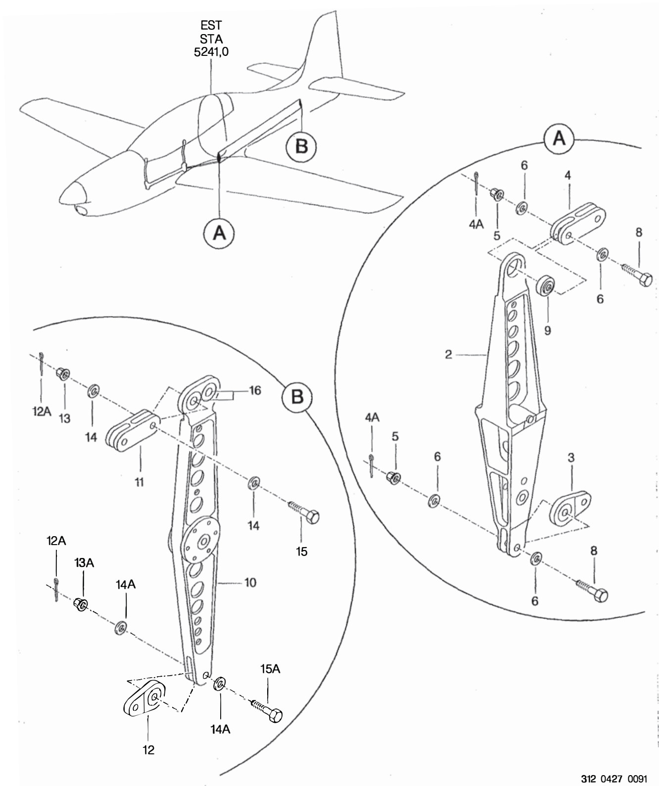
FIGURA 01. GUINHOIS DO PROFUNDOR CONJ FIGURE 01. ELEVATOR BELLCRANKS ASSY
