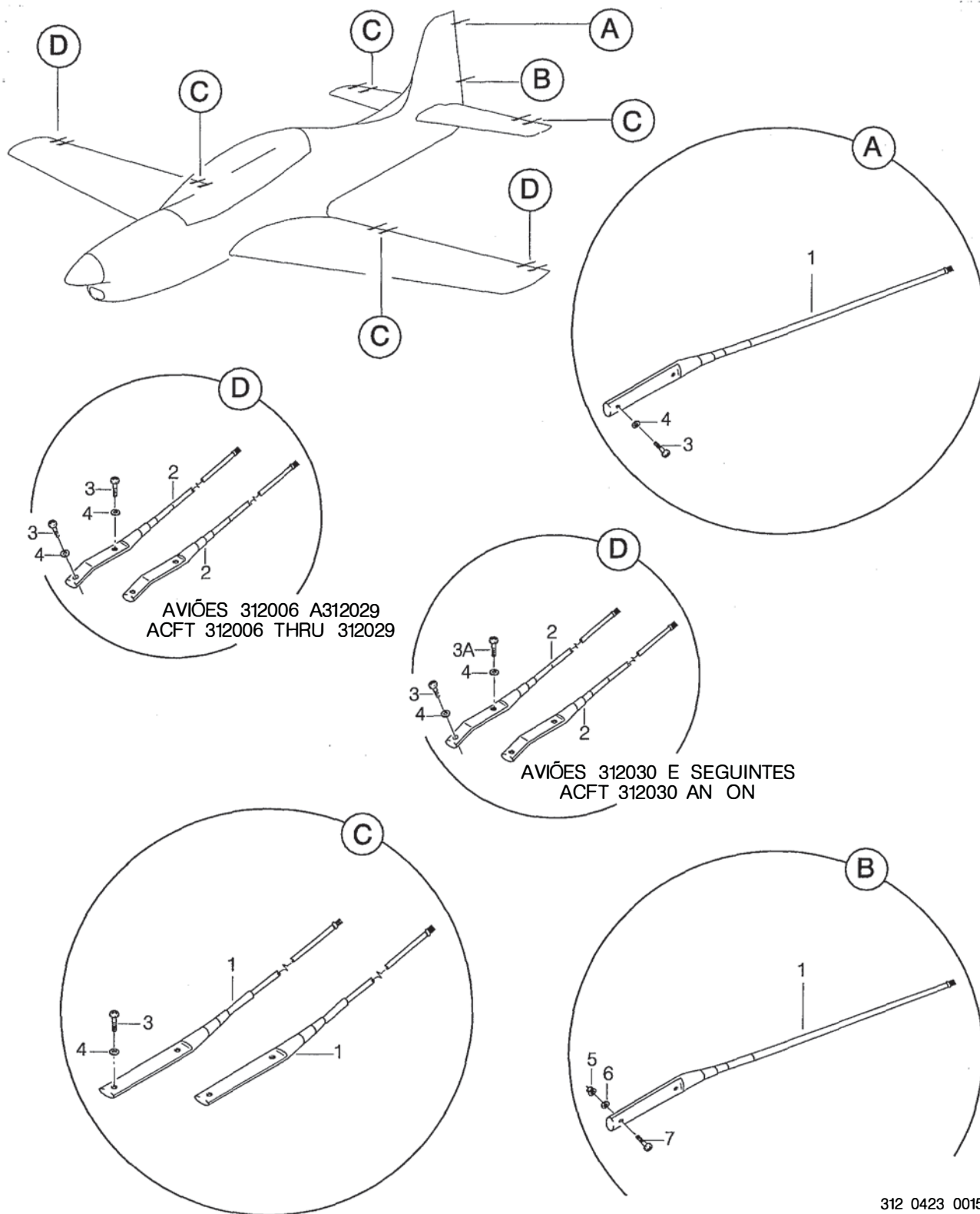
FIGURA 01. DESCARGA ESTATICA INSTL FIGURE 01. STATIC DISCHARGER INSTL
